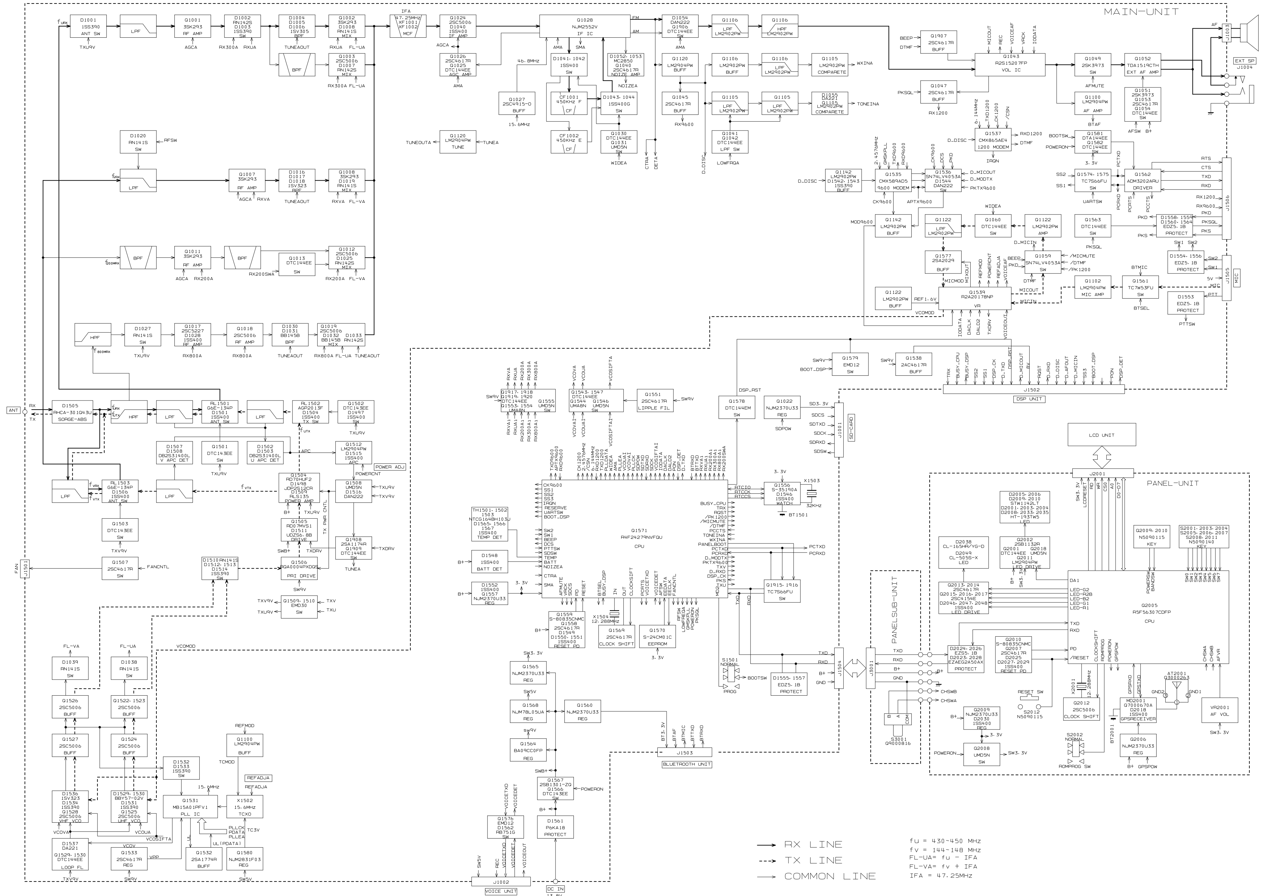
BLOCK DIAGRAM-1
