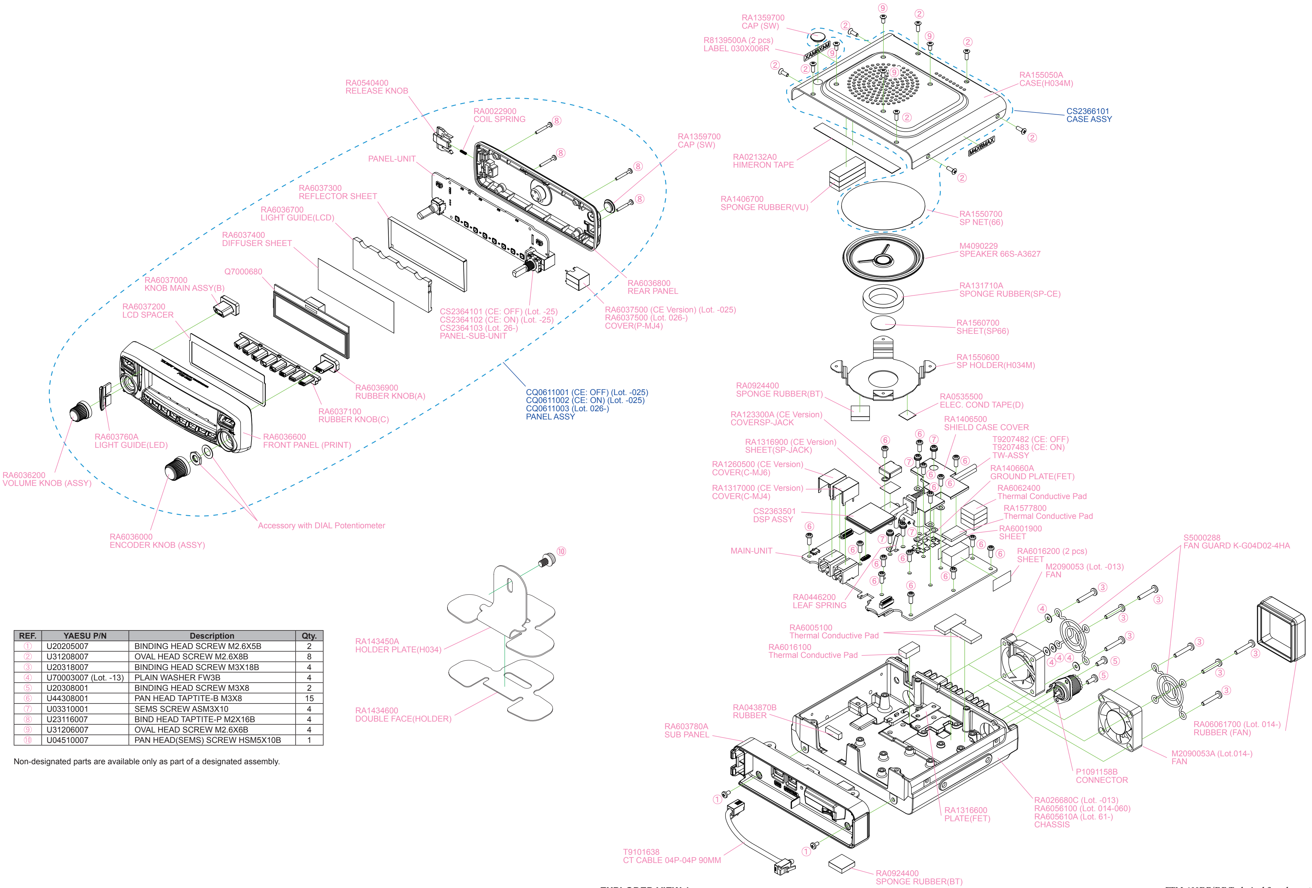
EXPLODED VIEW-1
