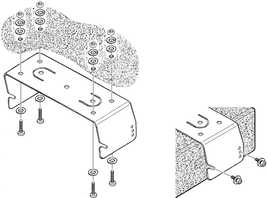
MMB-83 Installation
