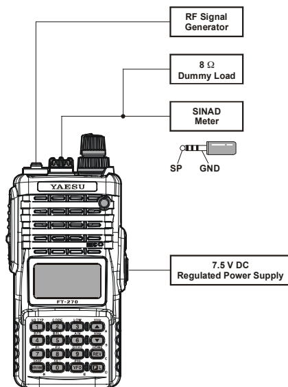
"RX SECTION" ALIGNMENT SETUP
