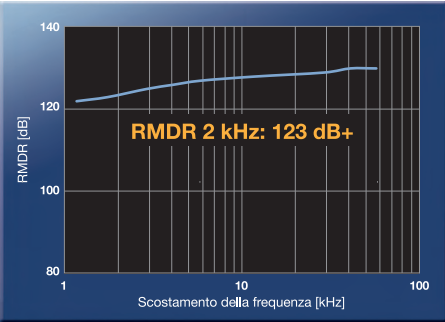
14 MHz Gamma dinamica reciproca al mixer Gamma dinamica (RMDR)
