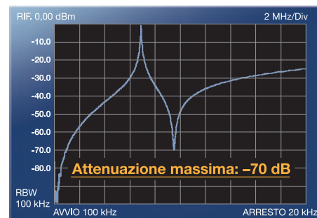
VC-Tune (7 MHz, intervallo 20 MHz)
