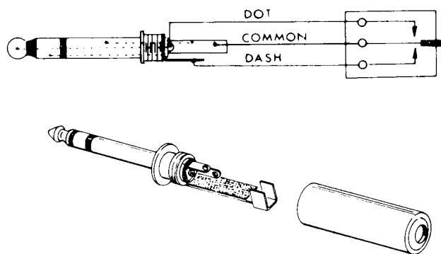
Keyer paddle plug connections
