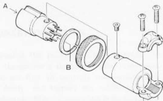
Plug assembly
