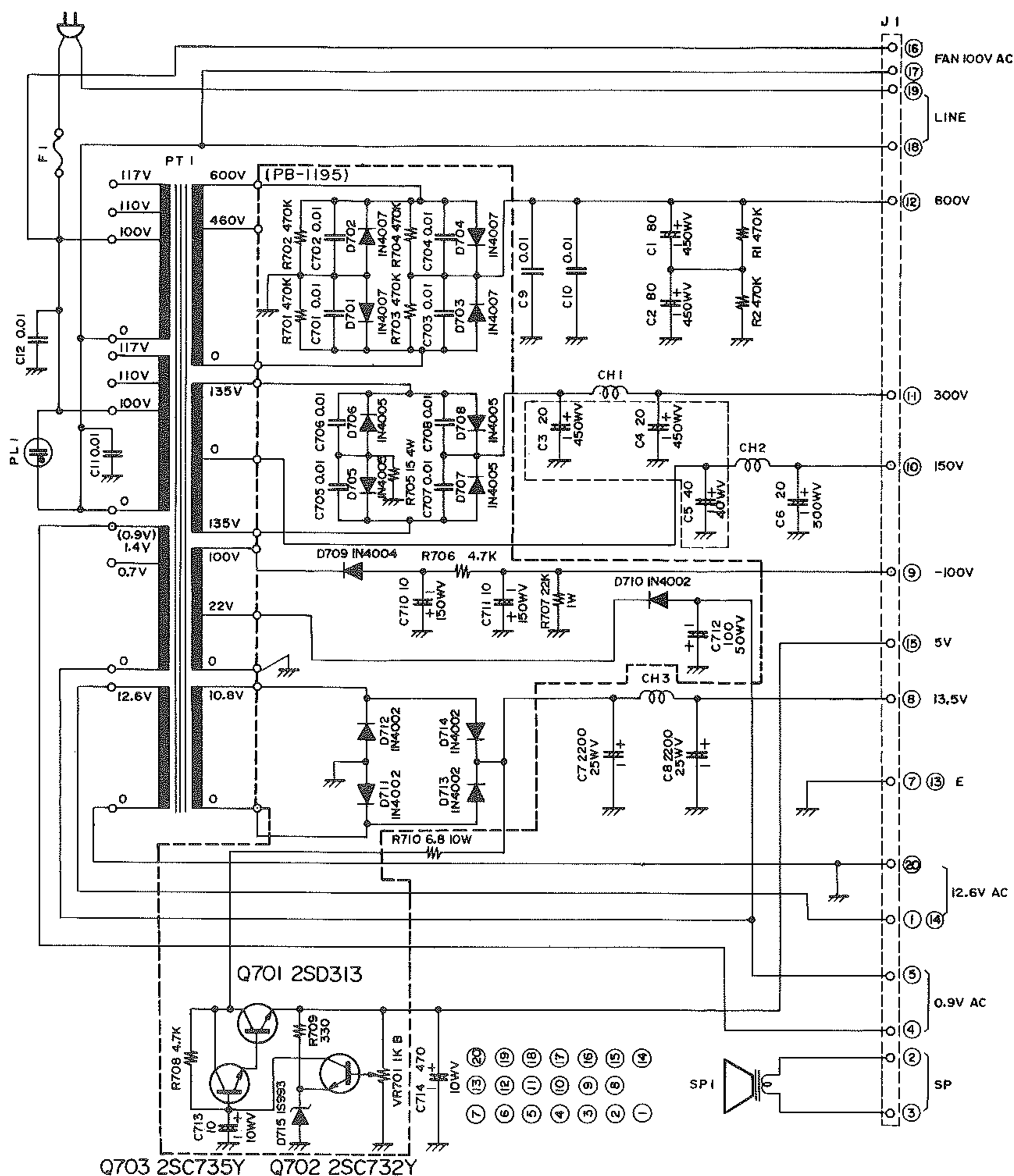
FP-501 CIRCUIT DIAGRAM
