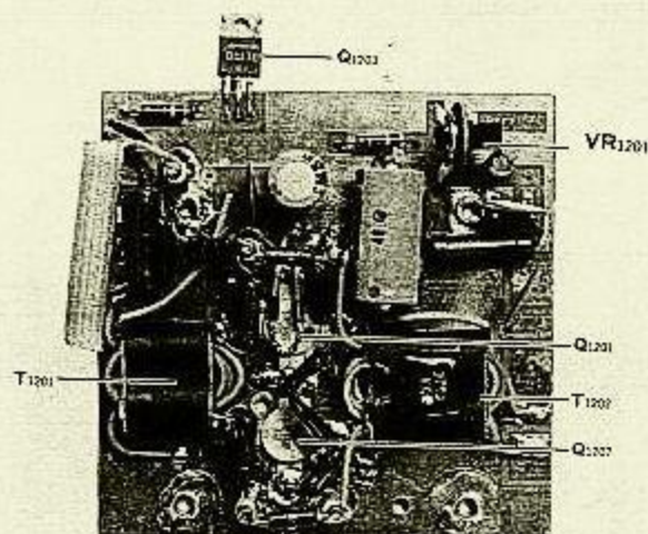
BOOSTER UNIT (PB-1444B)
