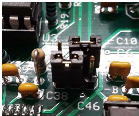
Jumpers installed for "USB" positions on J6
