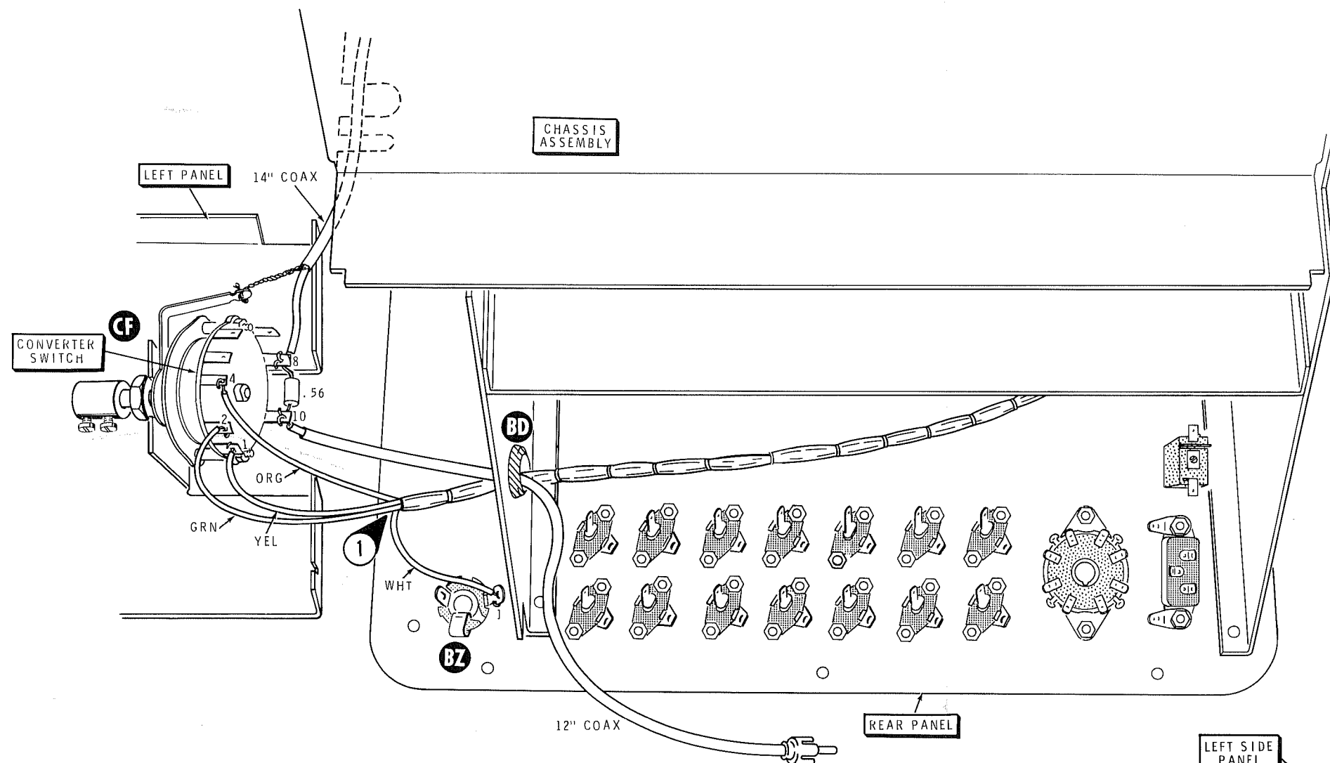
PICTORIAL 13-11
