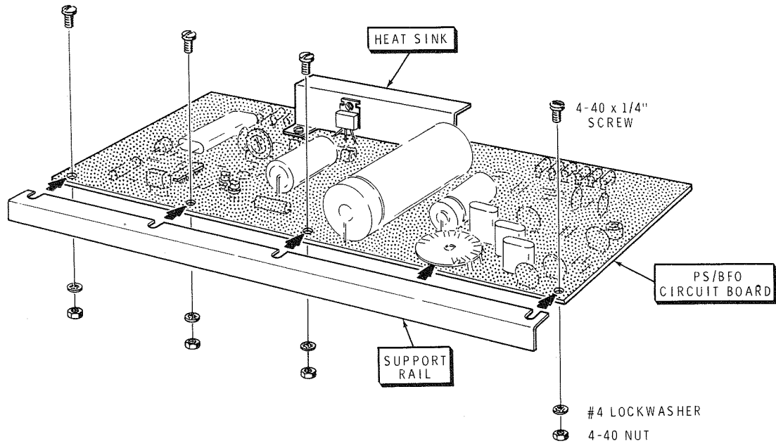
PICTORIAL 9-8
