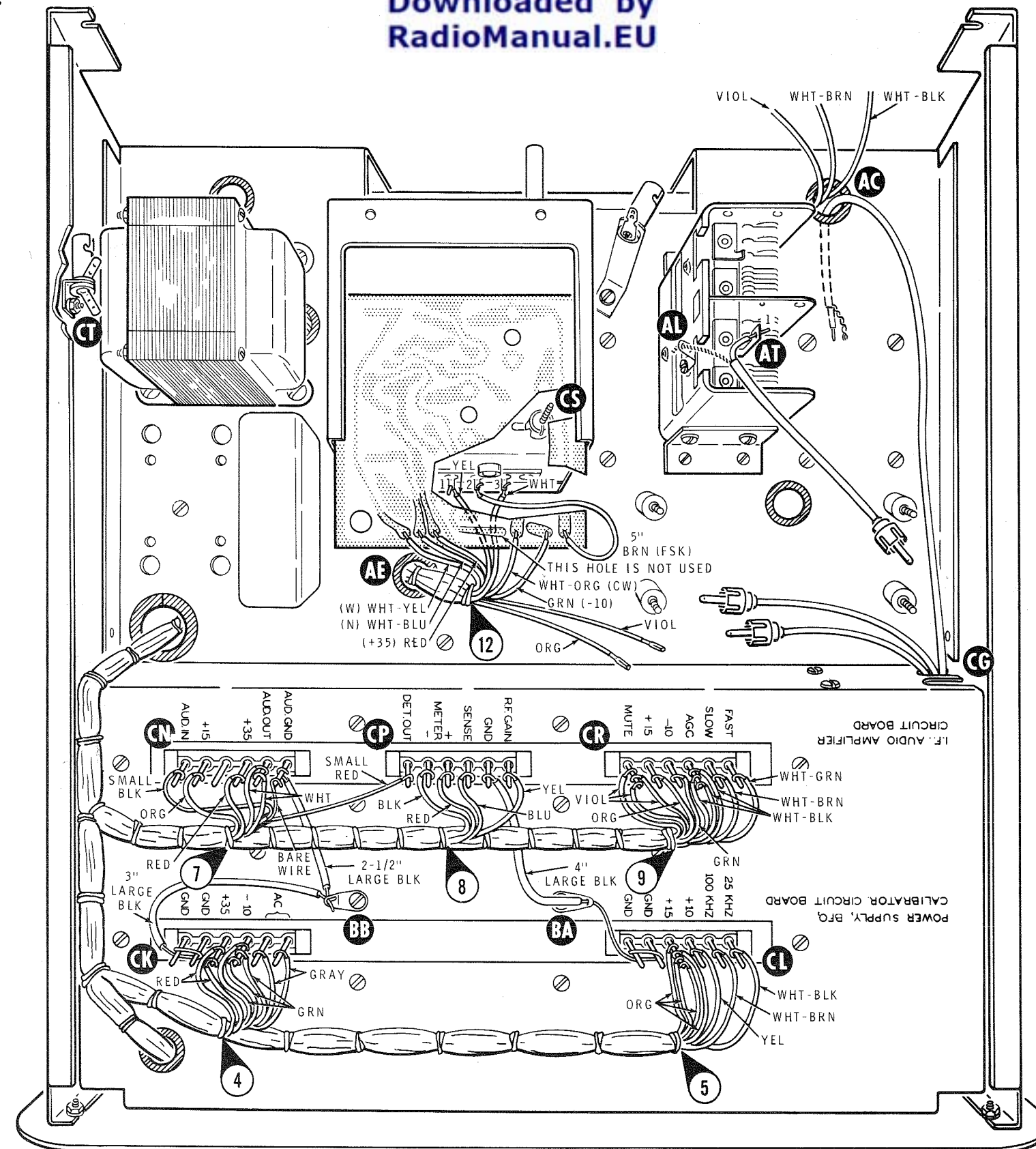
PICTORIAL 13-14
