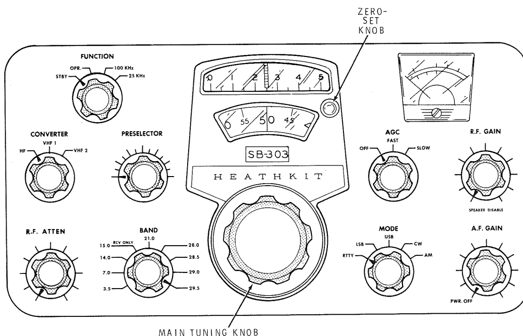
PICTORIAL 13-24
