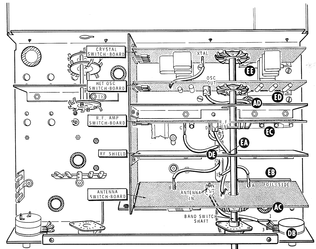
PICTORIAL 13-22
