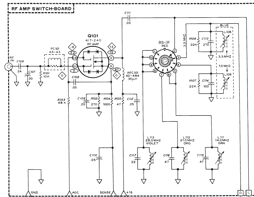
RF AMPLIFIER SWITCH-BOARD SCHEMATIC
