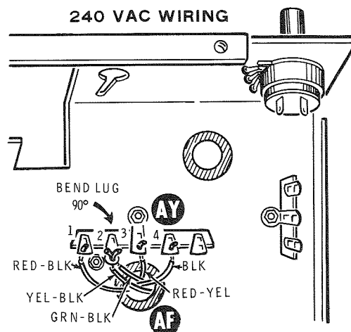
Detail 13-15D
