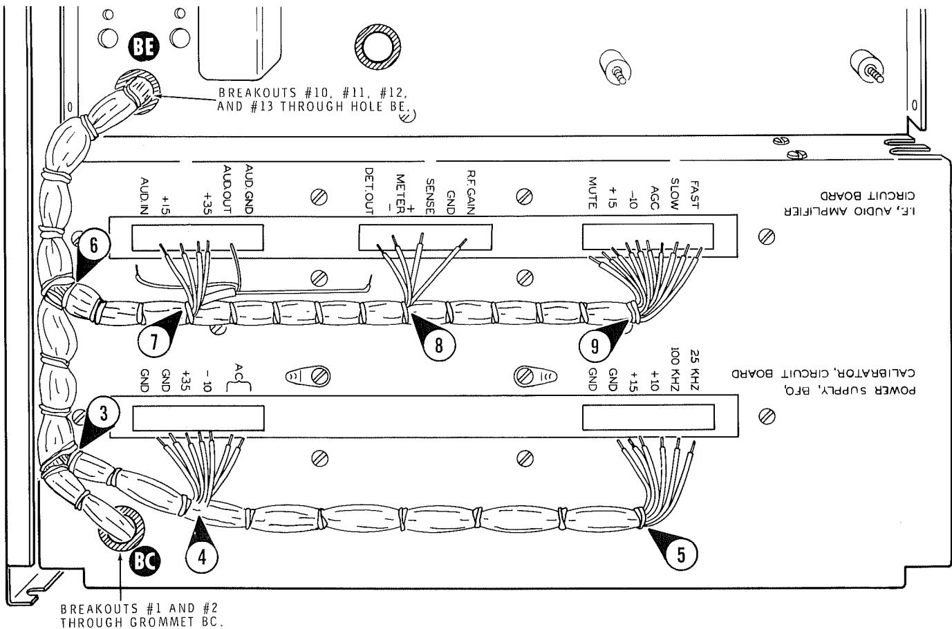
PICTORIAL 13-6
