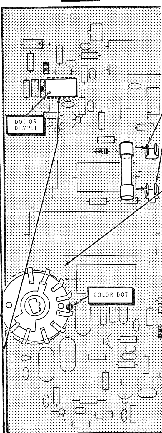
PICTORIAL 9-4
