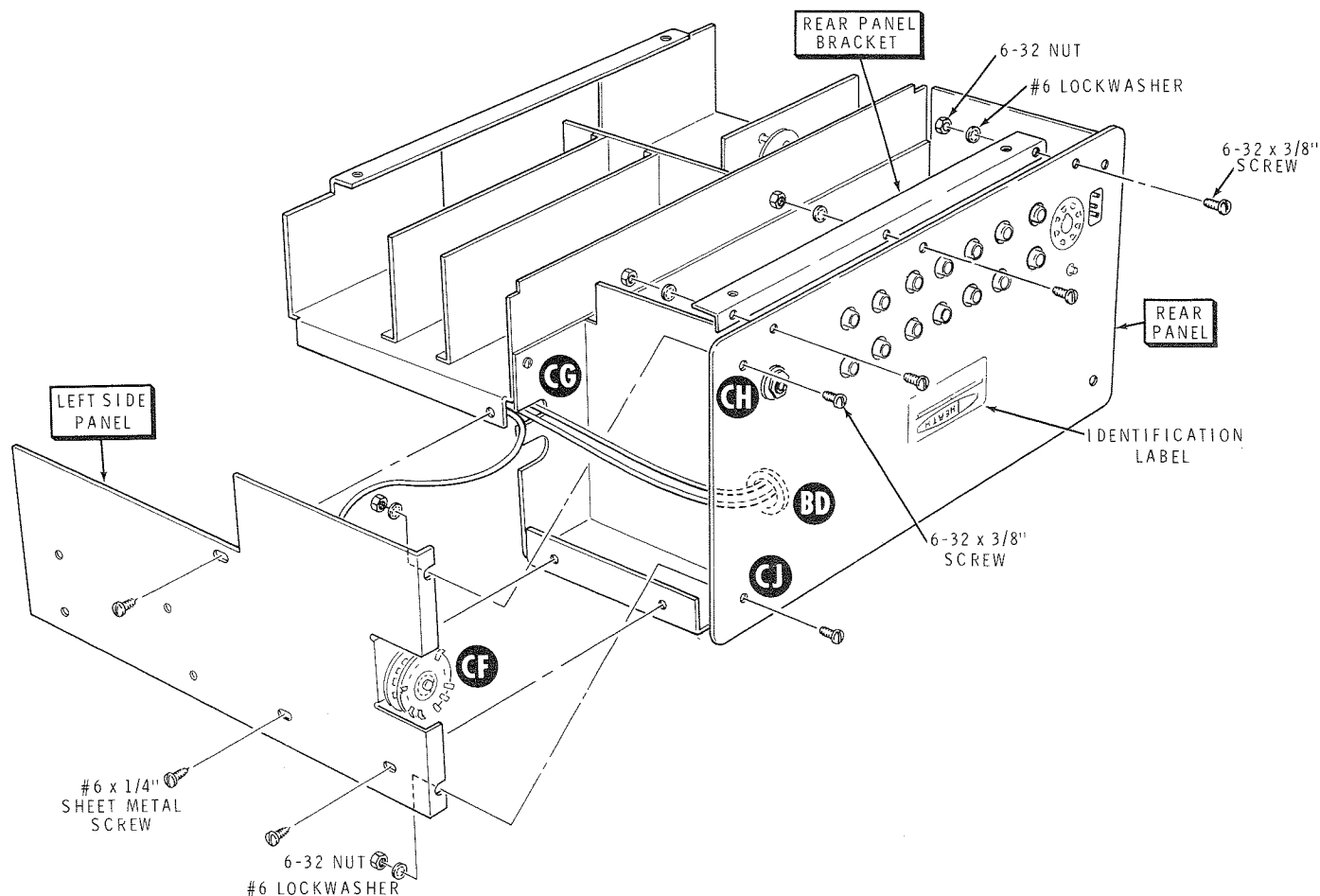
PICTORIAL 13-13
