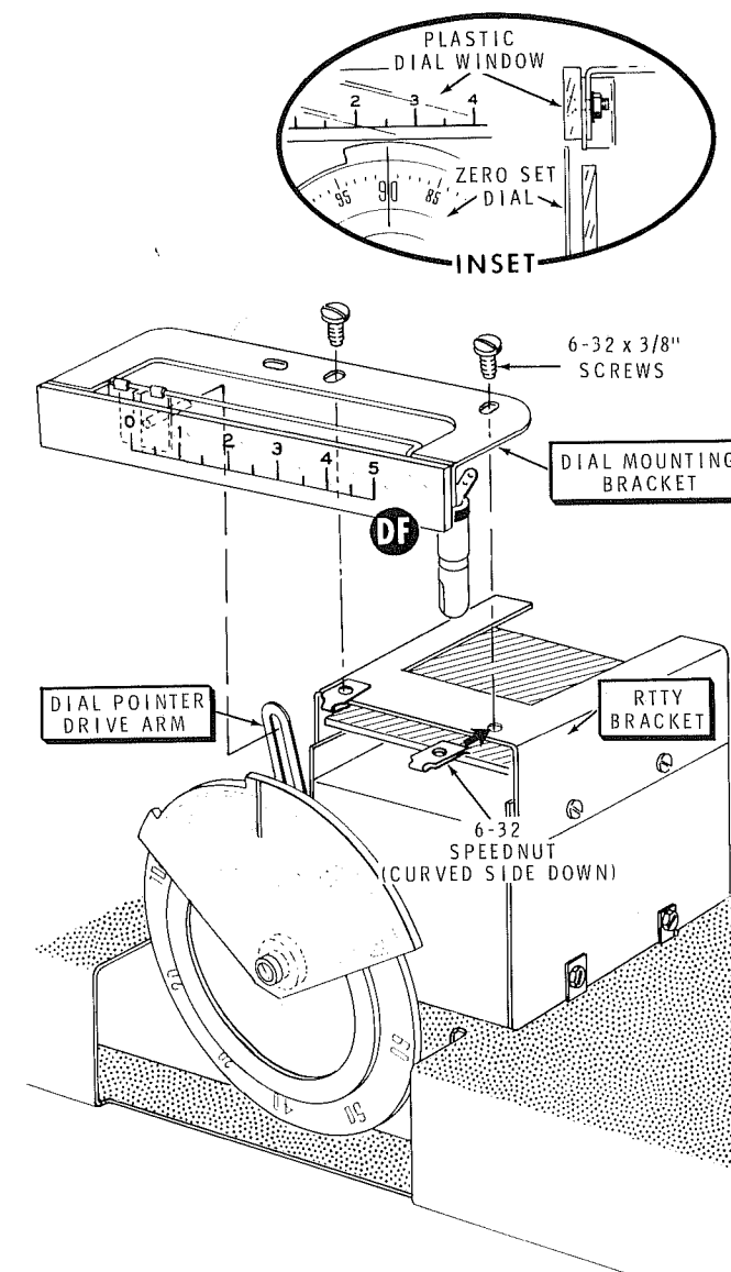
PICTORIAL 13-16
