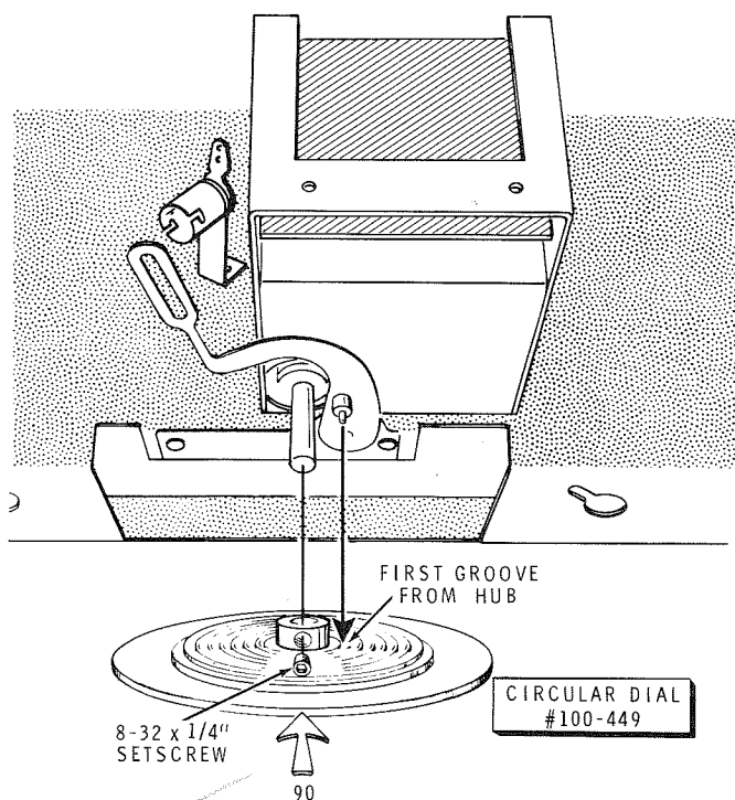
Detail 13-16C
