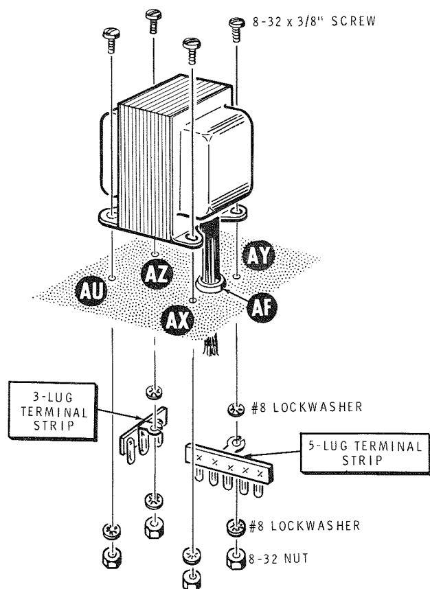
Detail 13-4G
