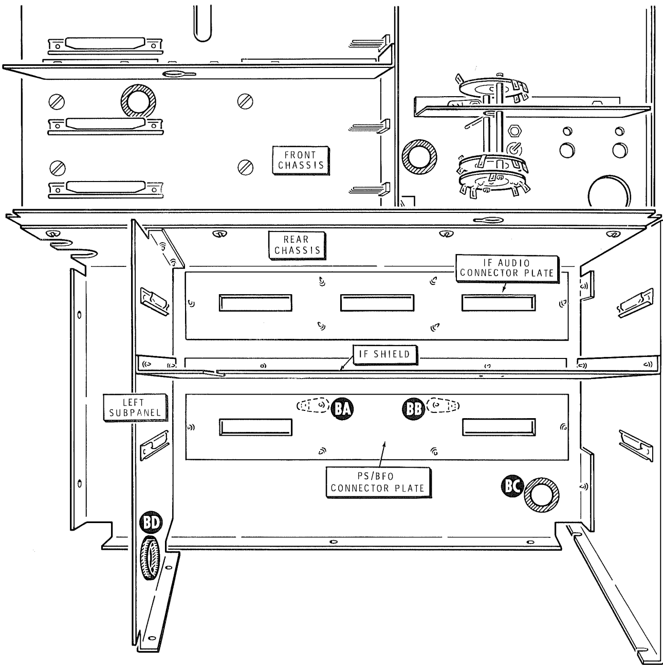
PICTORIAL 13-5
