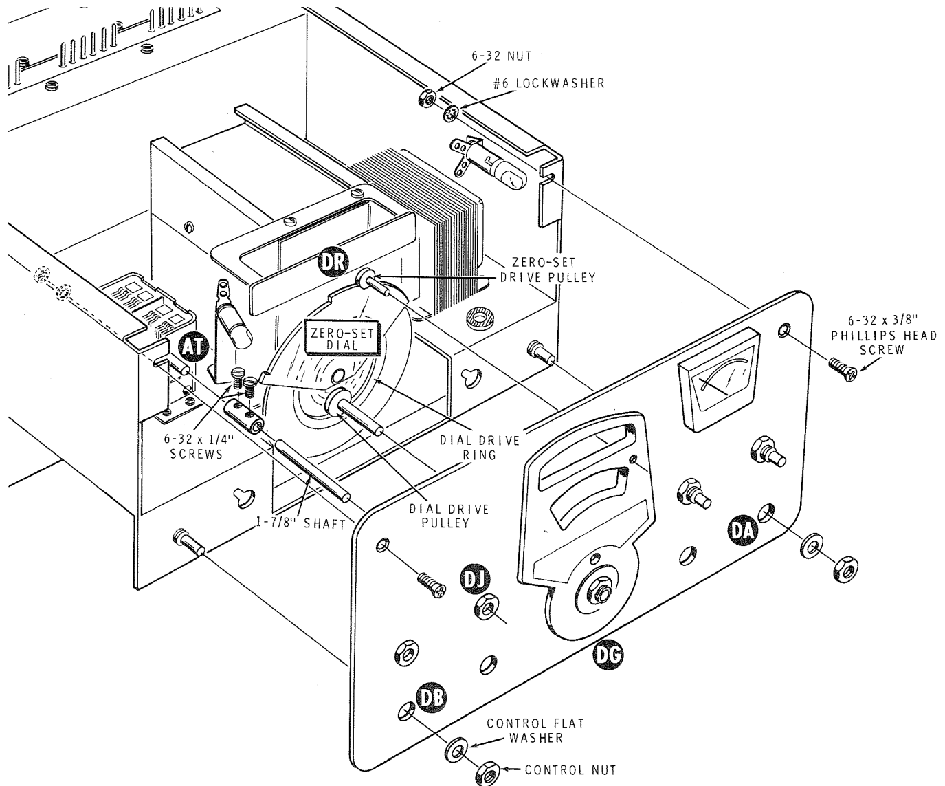
PICTORIAL 13-19
