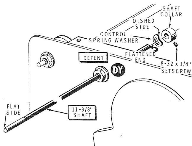
Detail 13-23C
