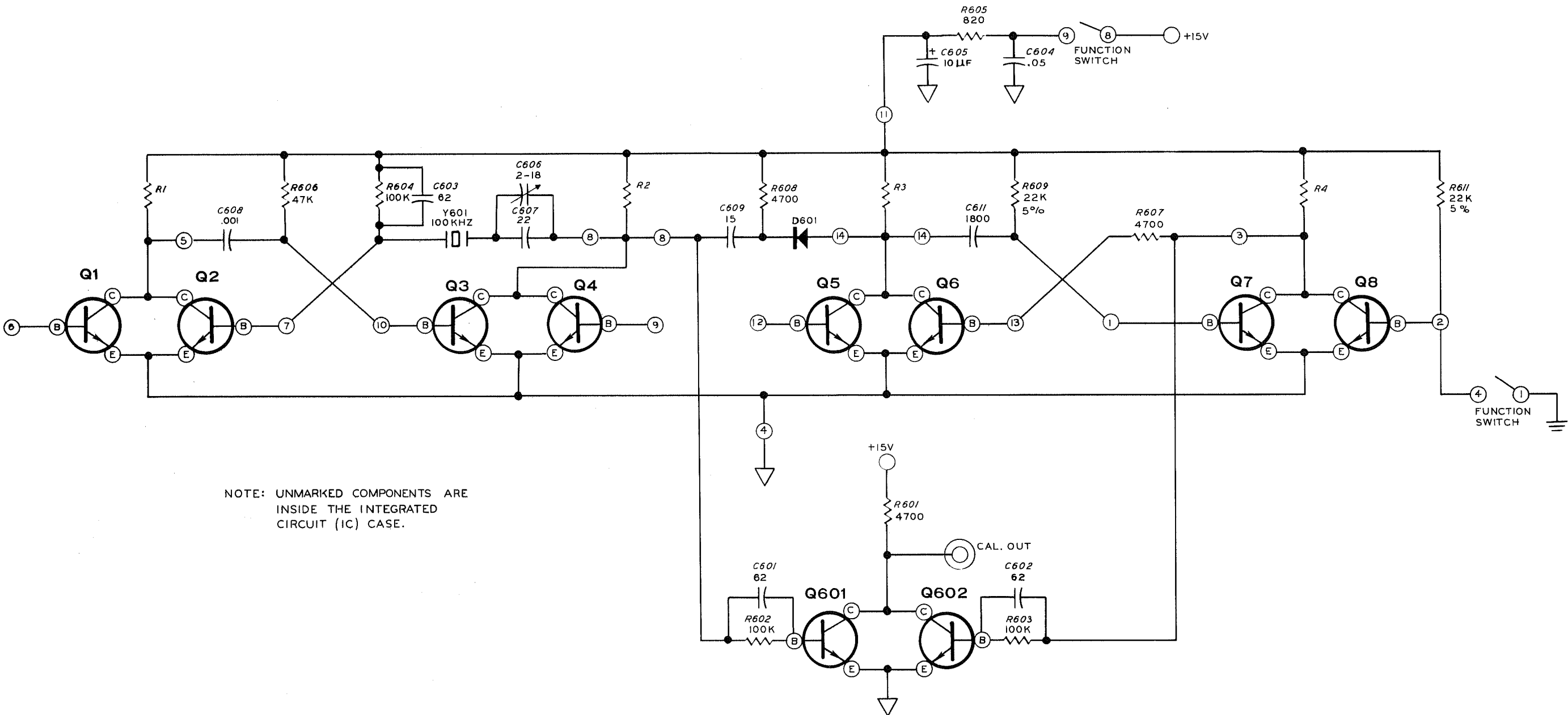
CALIBRATOR SCHEMATIC
