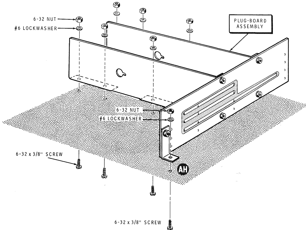
Detail 13-3B
