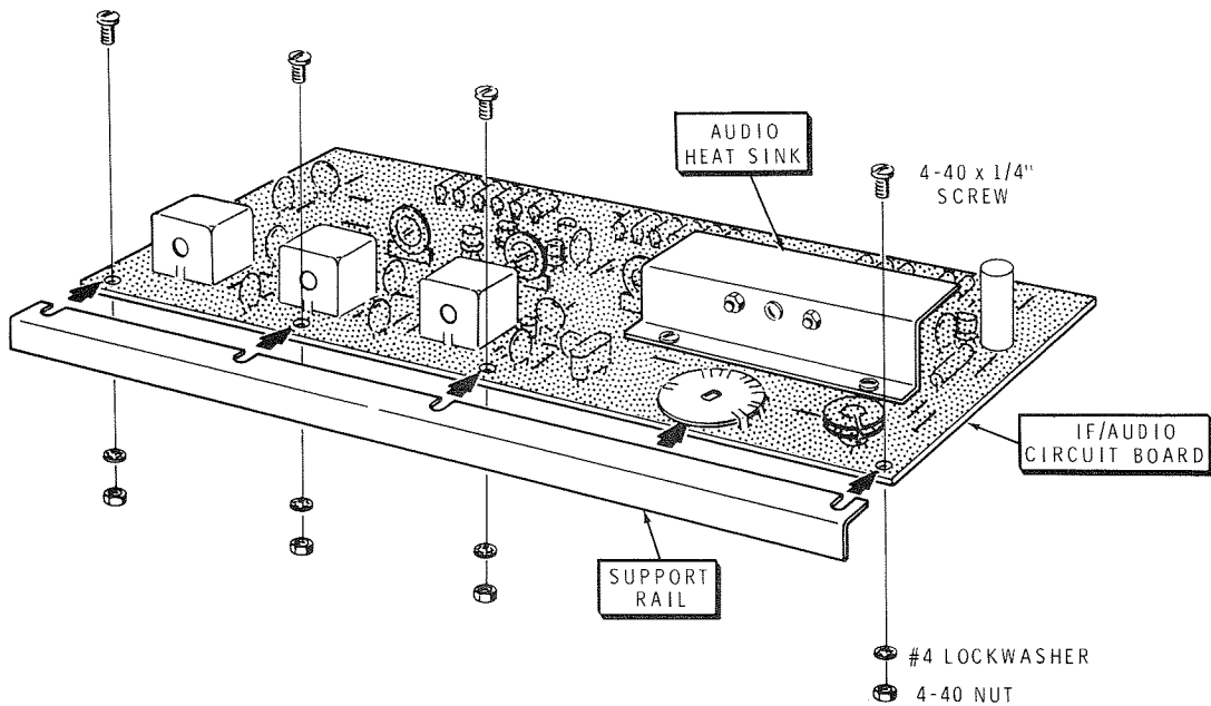
PICTORIAL 8-9
