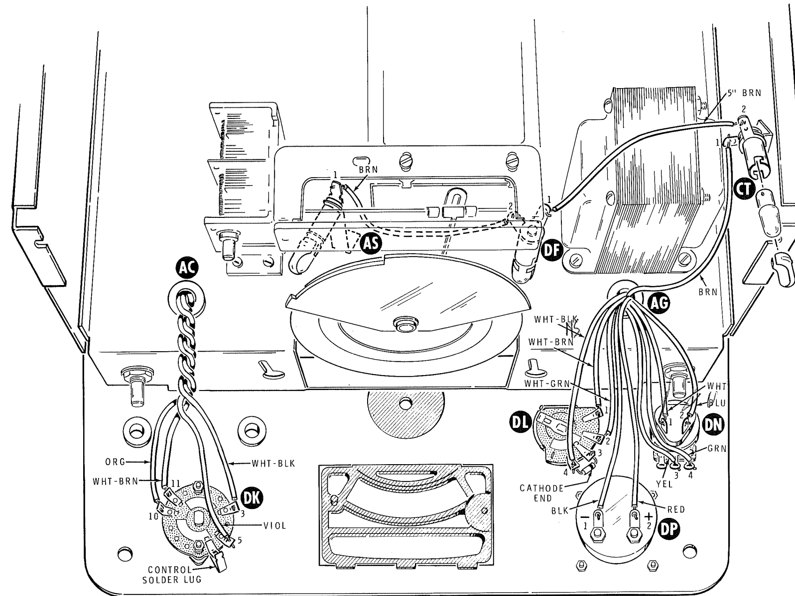
PICTORIAL 13-18
