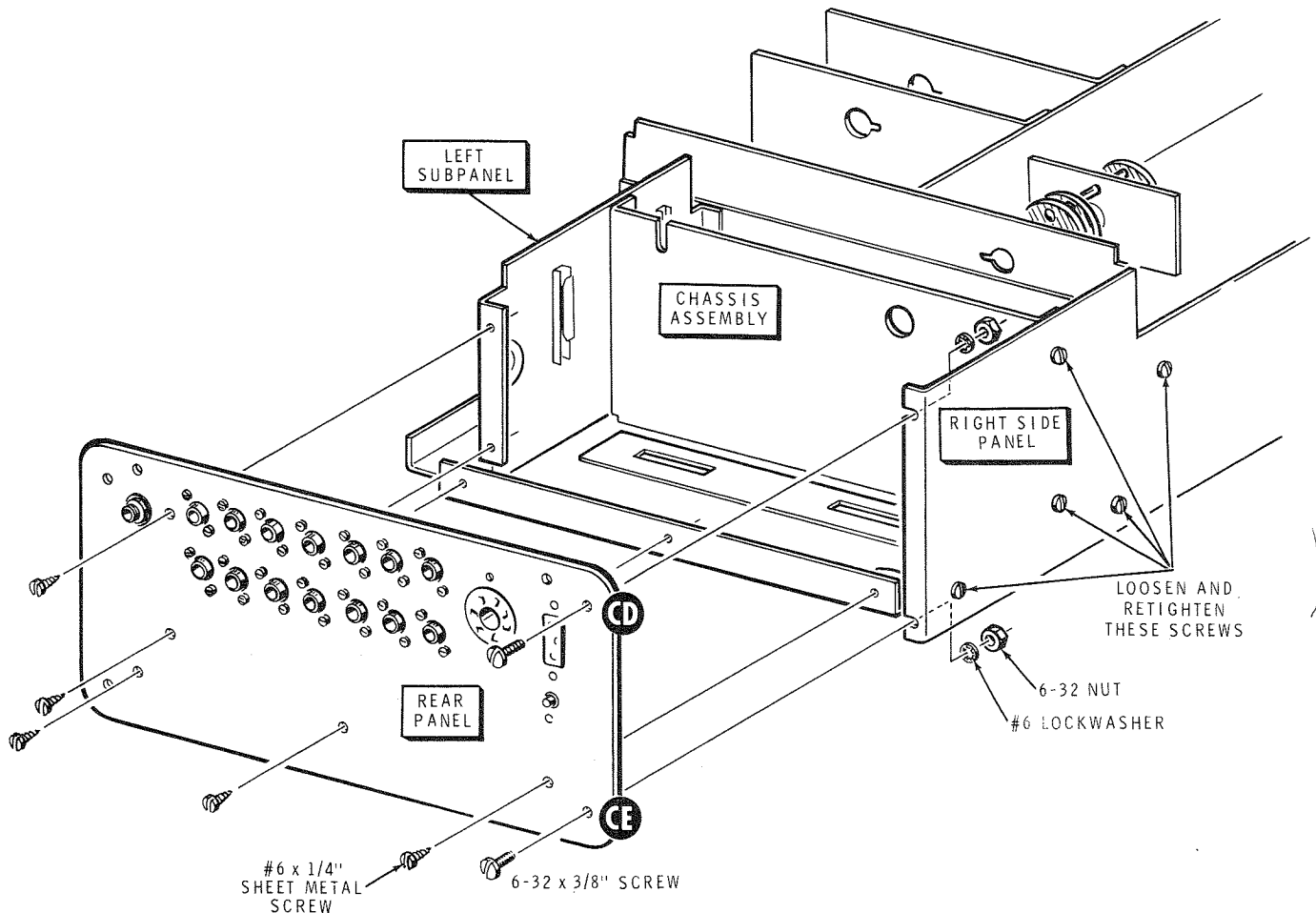
PICTORIAL 13-10
