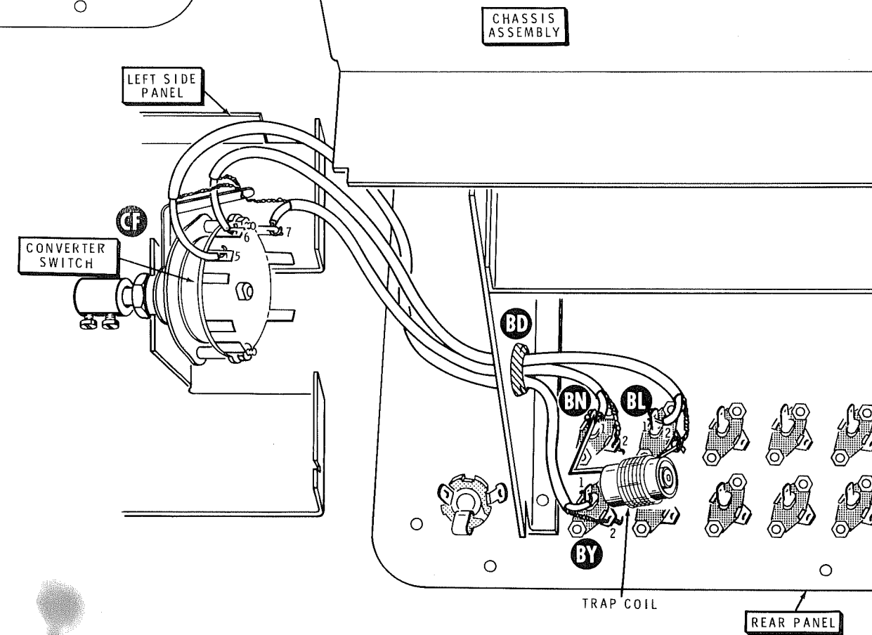
PICTORIAL 13-12
