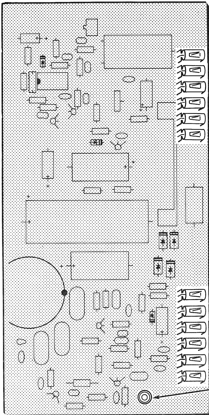
PICTORIAL 9-1
