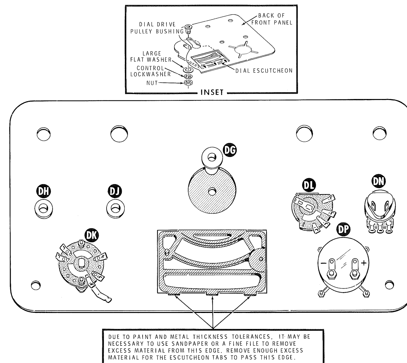
PICTORIAL 13-17
