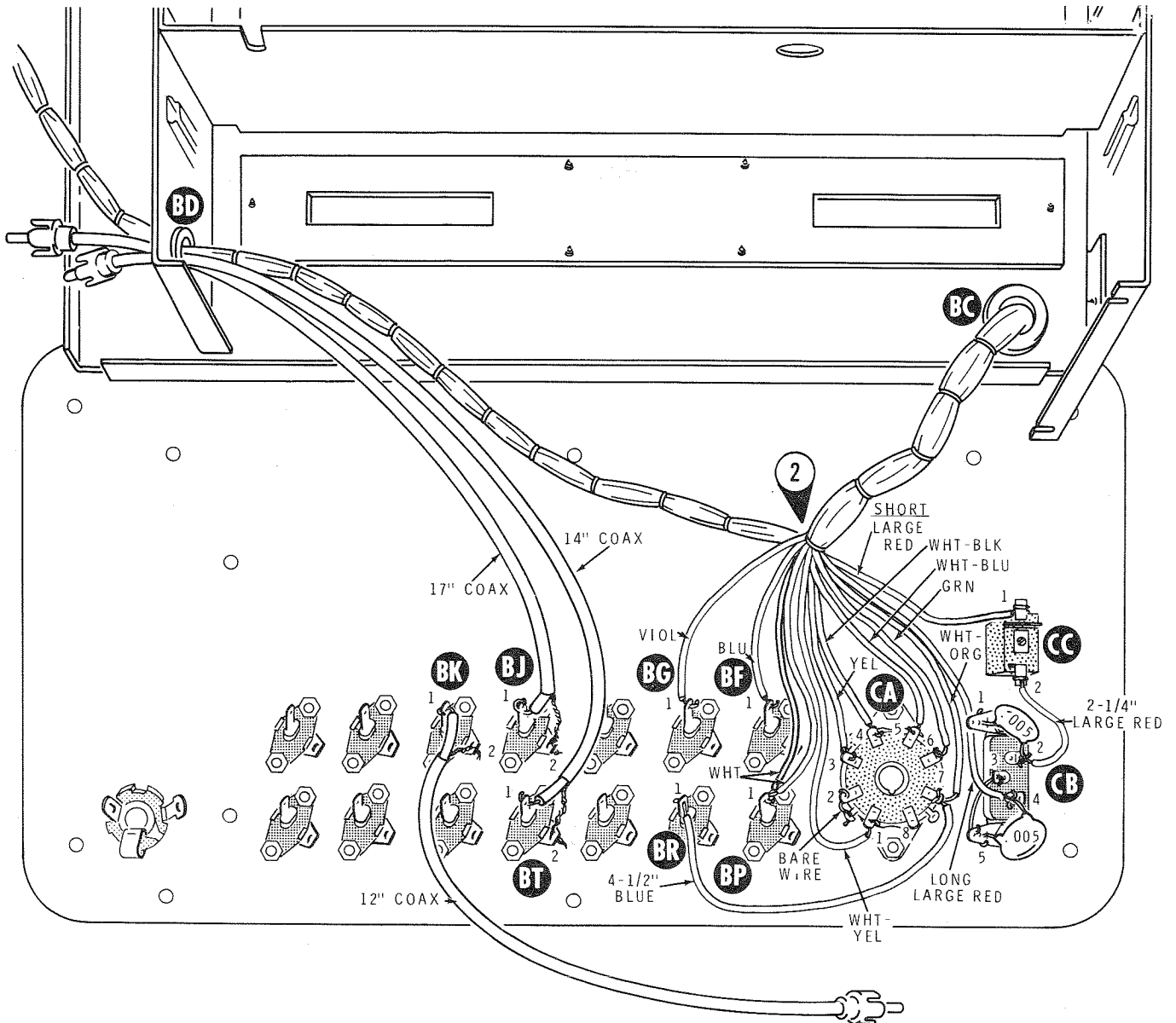
PICTORIAL 13-9
