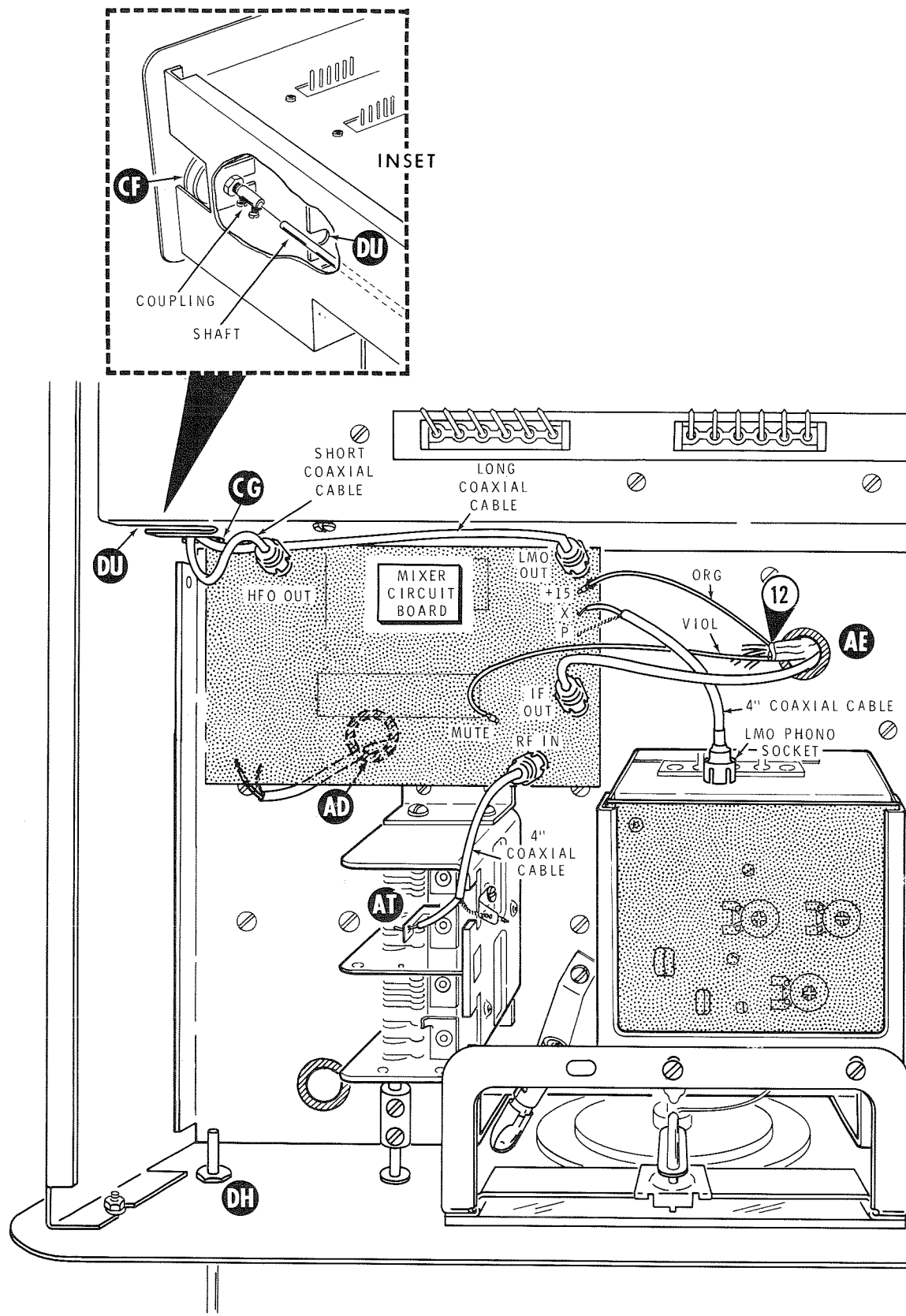
PICTORIAL 13-20
