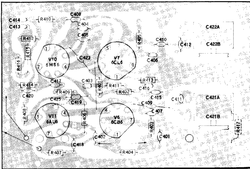
RF-DRIVER CIRCUIT BOARD #85-131-5
