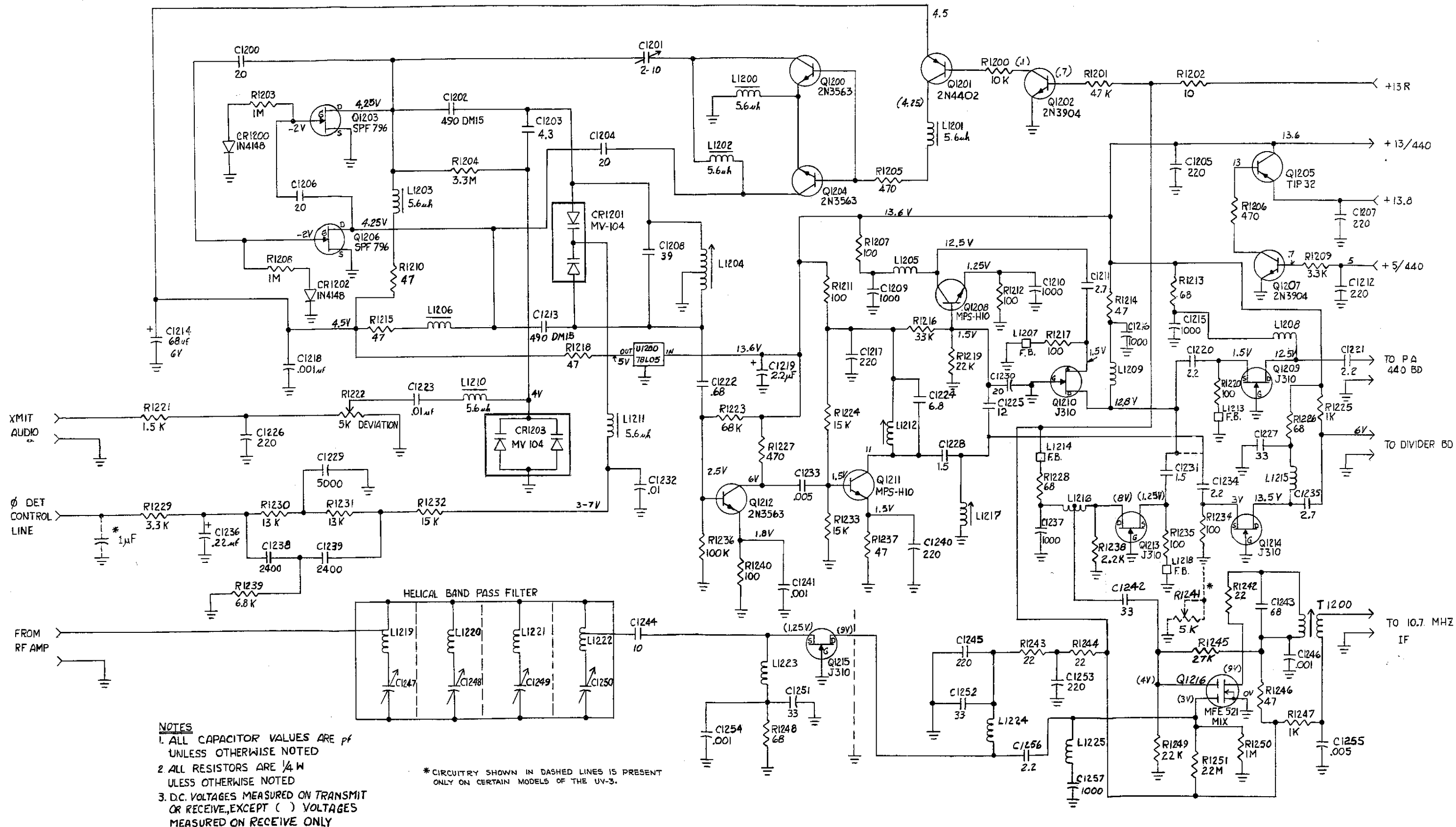
FIGURE 2-5. 440 MHz RECEIVER/VCO SCHEMATIC
