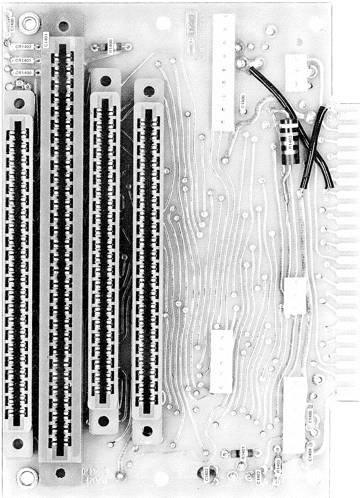
FIGURE 11-1. PARENT BOARD
