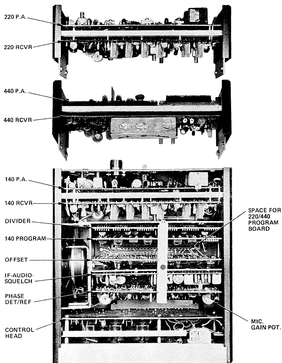
FIGURE 1-1. BOARD LOCATIONS
