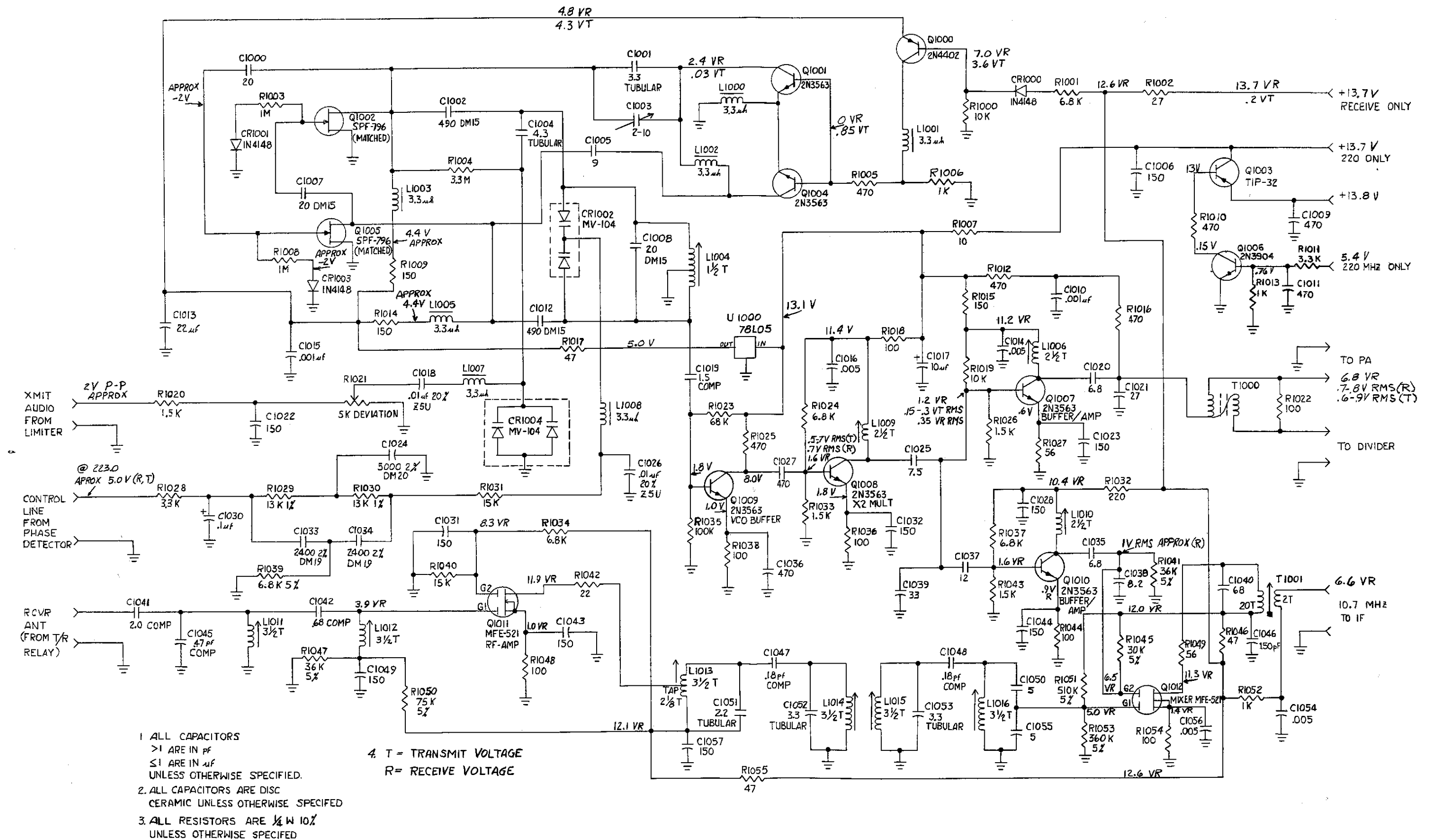
FIGURE 2-3. 220 MHz RECEIVER/VCO SCHEMATIC
