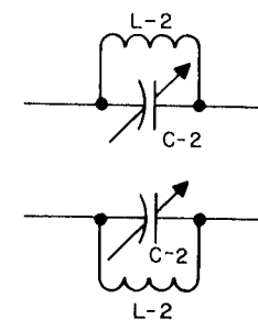
144 mc TRAP
