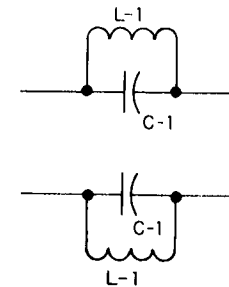
50 mc TRAP
