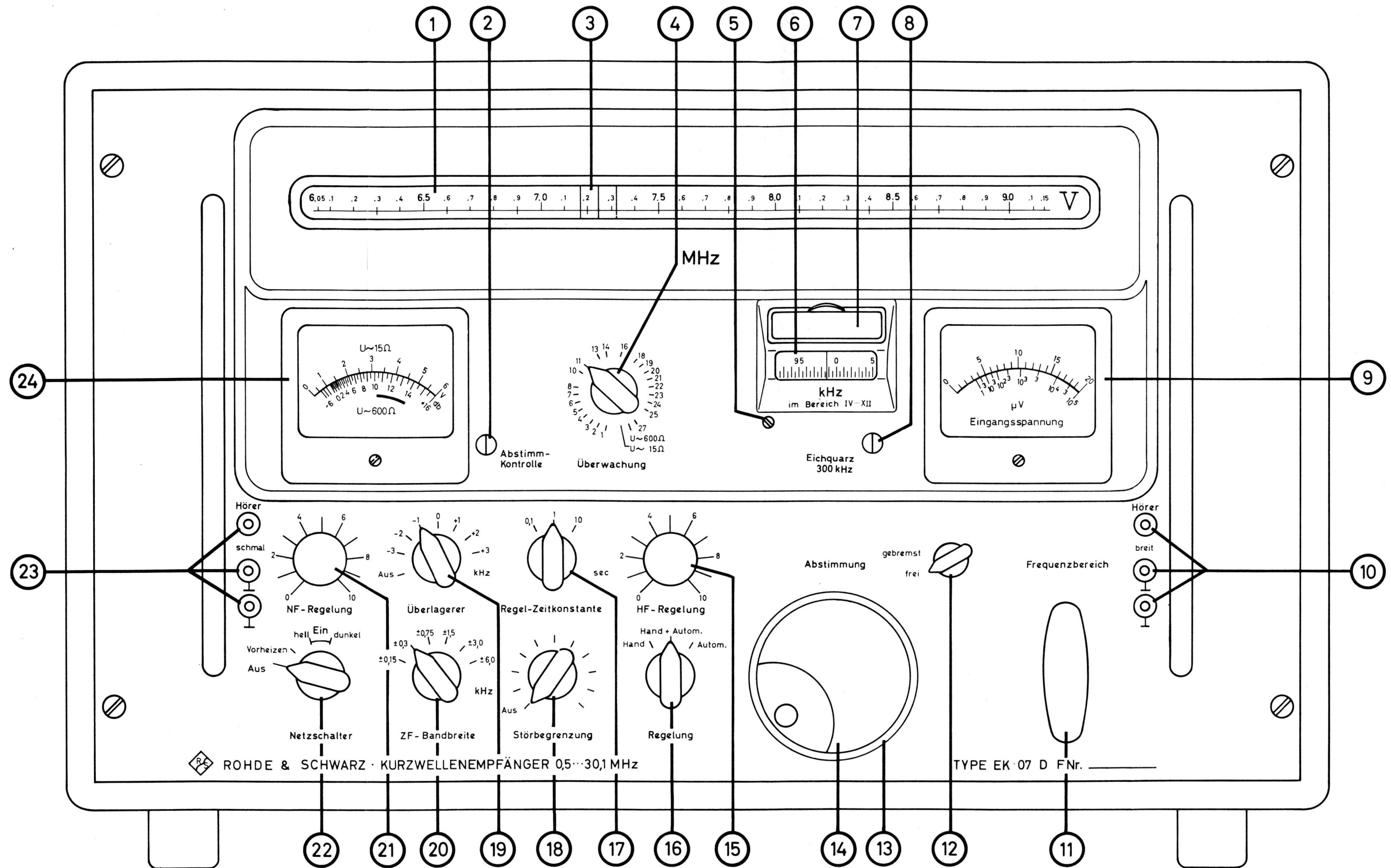
Front Panel
