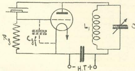
FIG. 59.—Pierce oscillator.
