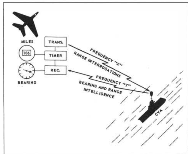
Figure 9-10.—Dual-frequency transmission.
