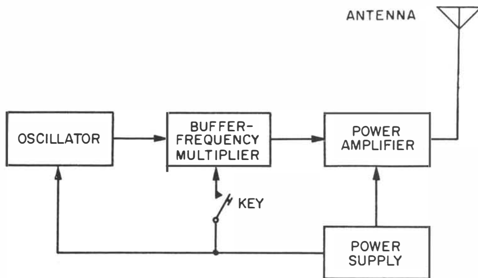
Figure 2-2.—Continuous-wave transmitter.
