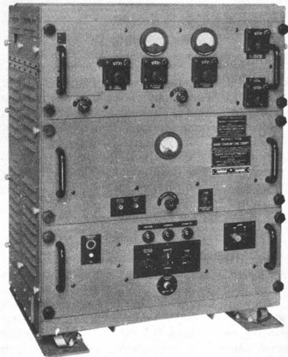
Figure 3-11.—VHF transmitter model TDQ.
