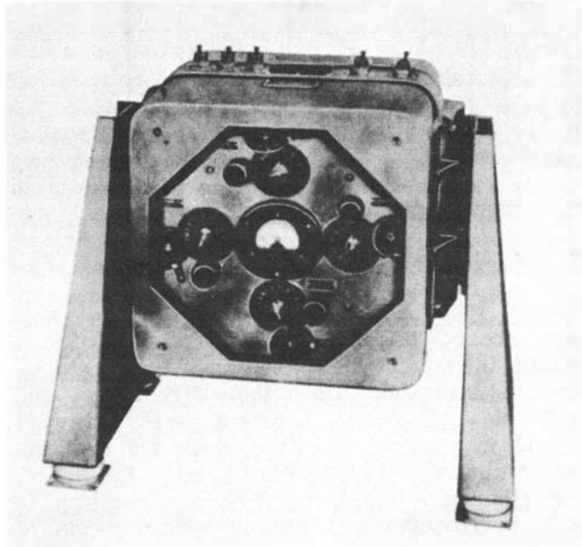
120.13 Figure 3-43.—VHF-UHF antenna multicoupler CU-274/UR.
