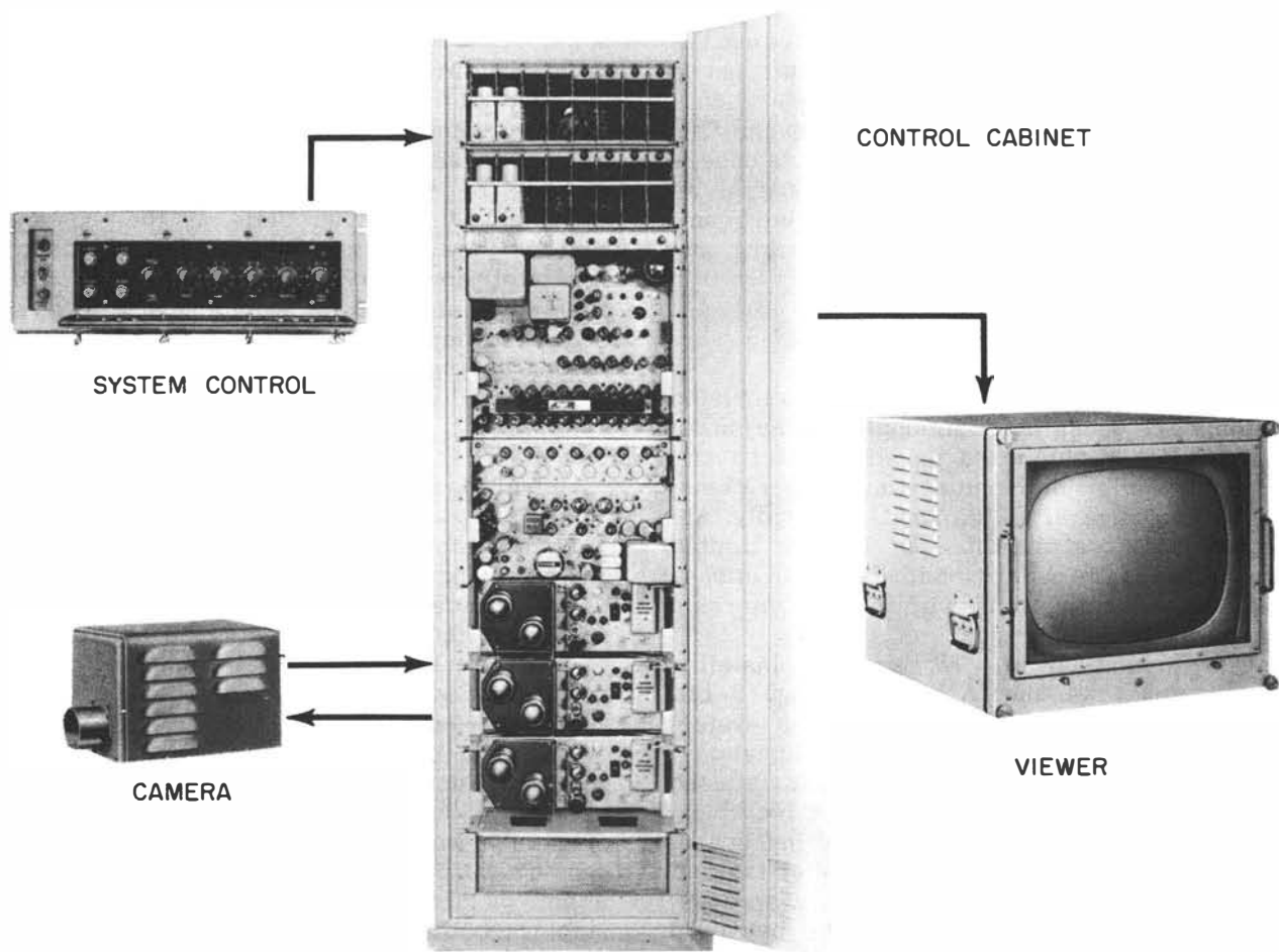
Figure 9-14.—Television system AN/SXQ-2.
