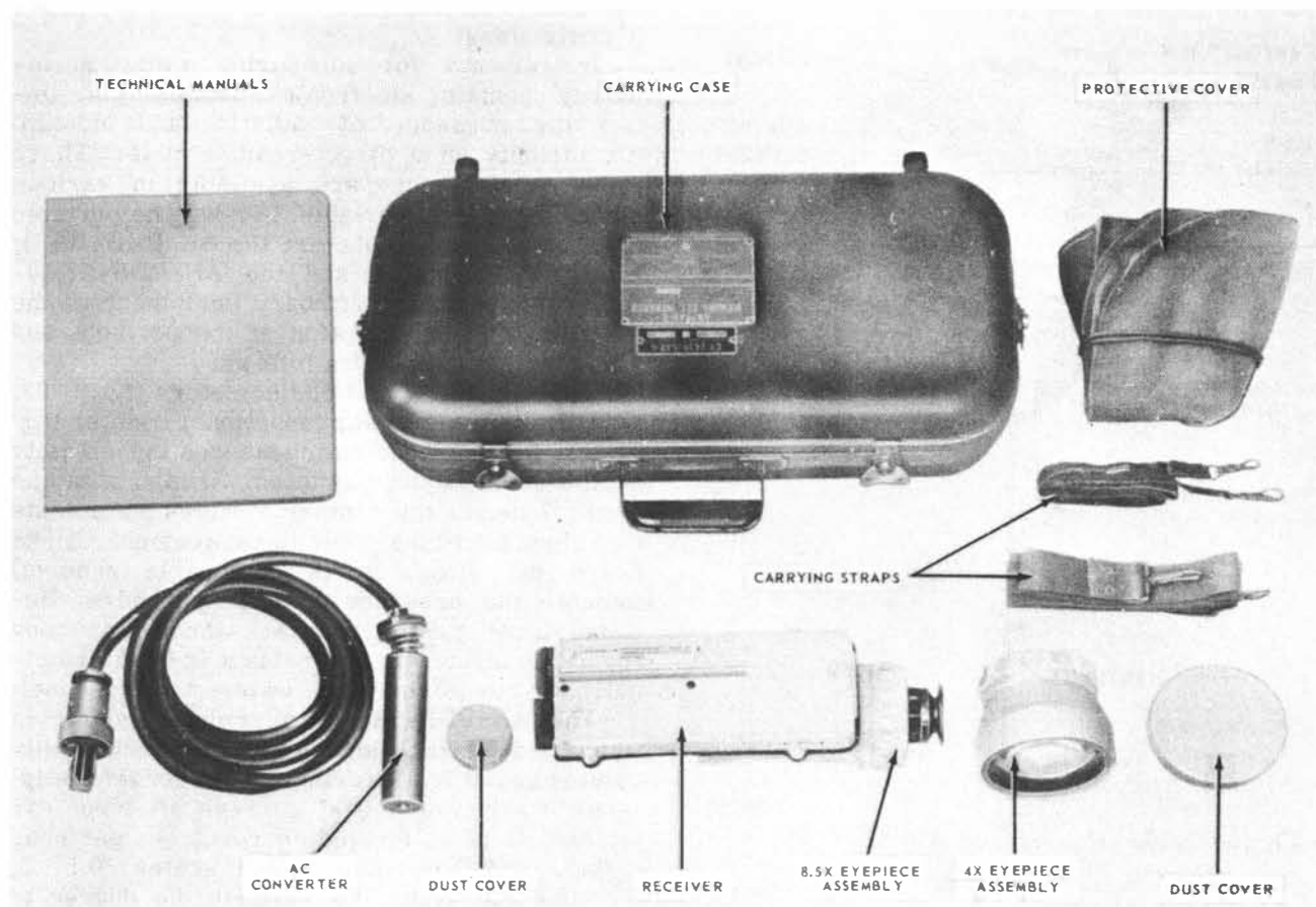
Figure 9-19.—Electronic infrared receiver AN/SAR-6.
