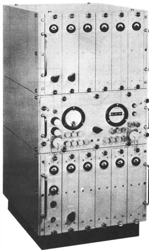
31.37 Figure 4-25.—Telegraph terminal set AN/UGC-1( ).
