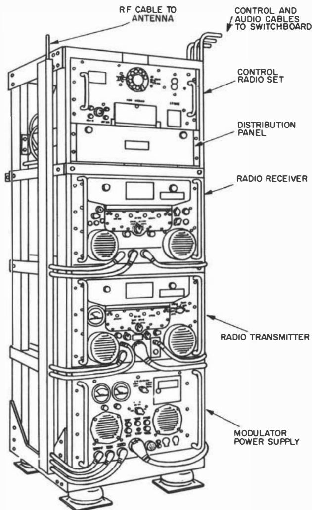
Figure 3-13.—Transmitter-receiver AN/GRC-27( ).
