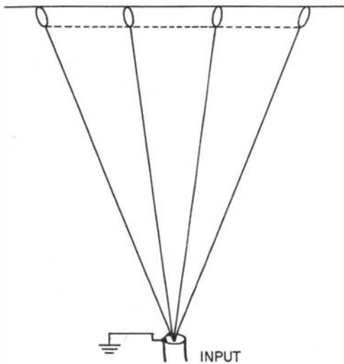
Figure 3-34.—Fan antenna.
