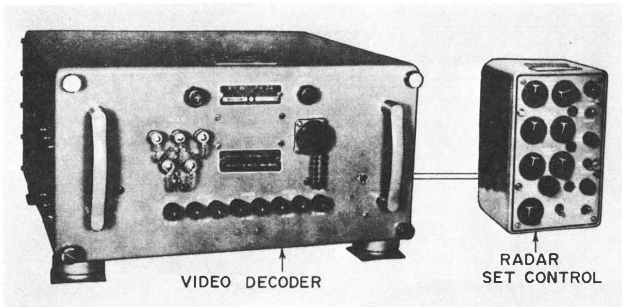
Figure 6-11.—Decoder Group AN/UPA-24( ).
