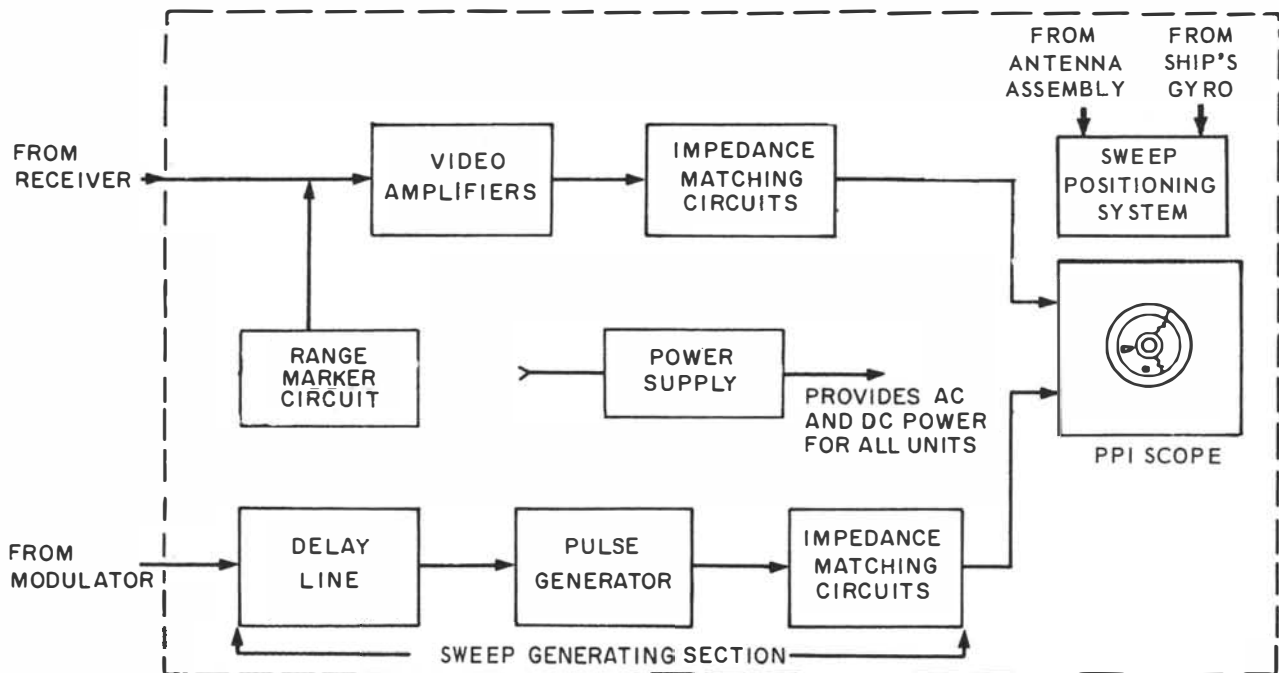
Figure 5-10. —Radar indicator.
