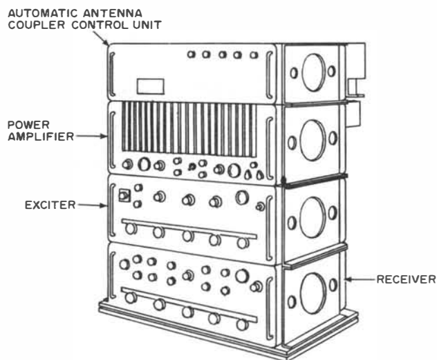
Figure 3-6.—Radio set AN/WRC-1.
