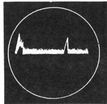
Figure 5-11.—A-scope presentation.
