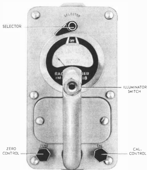
Figure 9-24.—Radiacmeter AN/PDR-18( ), 100.128
