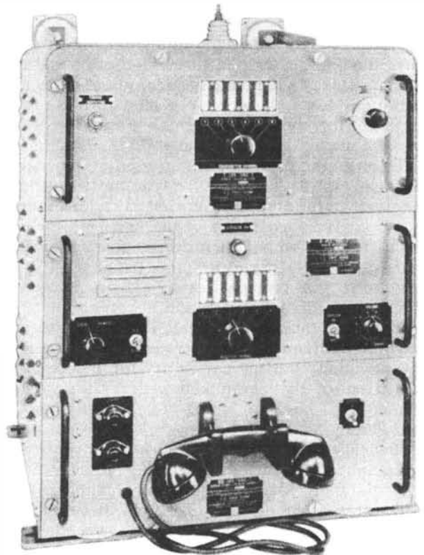
Figure 3-2.—Transmitter-receiver 76.19 AN/URC-7.
