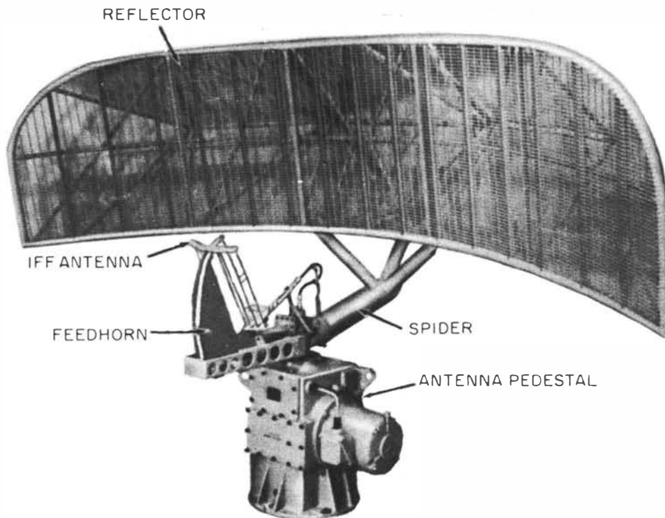
Figure 5-17.—Barrel stave antenna. 32.186
