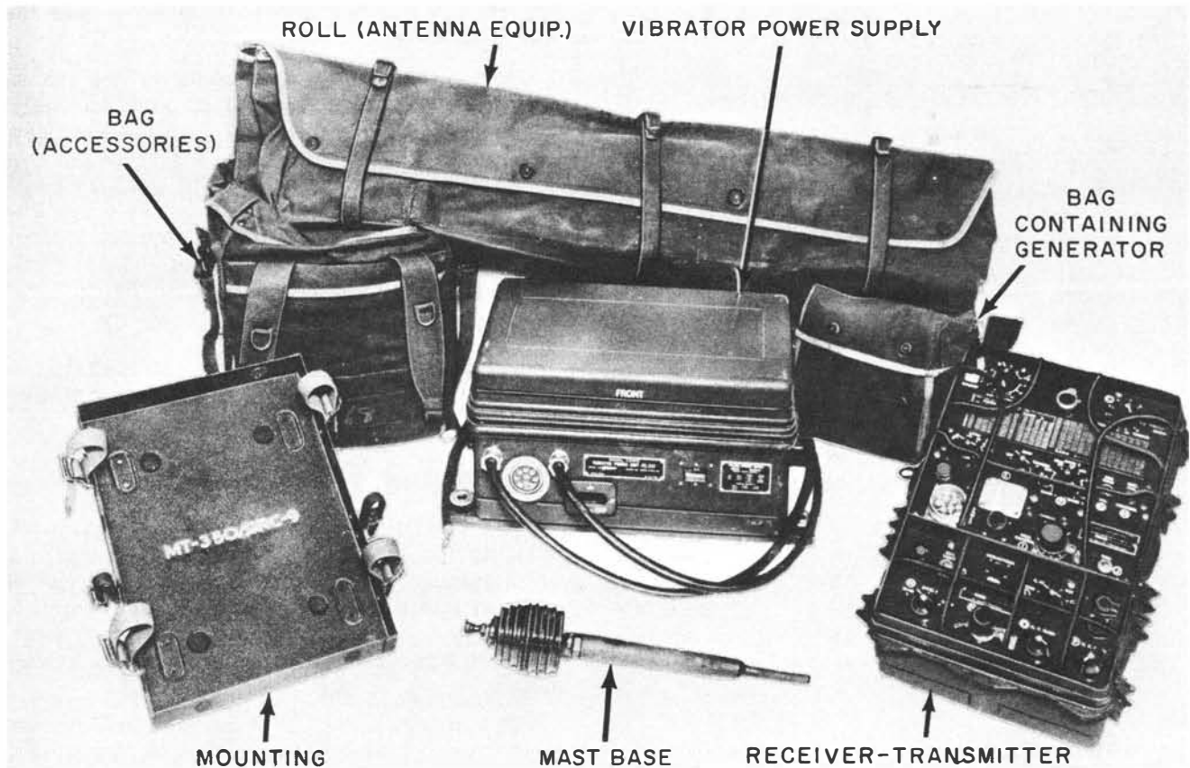
Figure 3-15.—Radio set AN/SRC-9( ).
