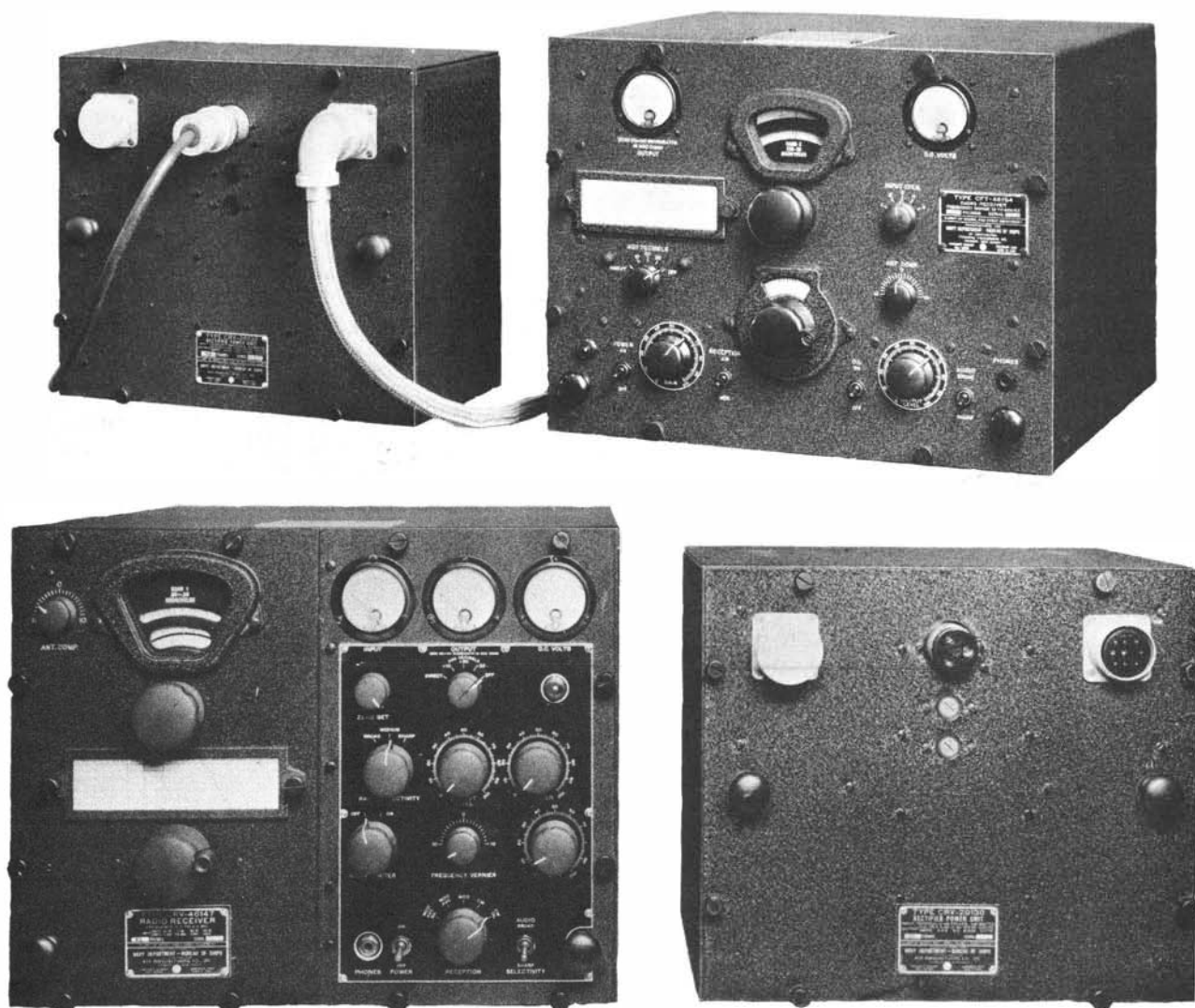
Figure 3-26.—Receivers with power supply; top, model RBA; bottom, models RBB/RBC.
