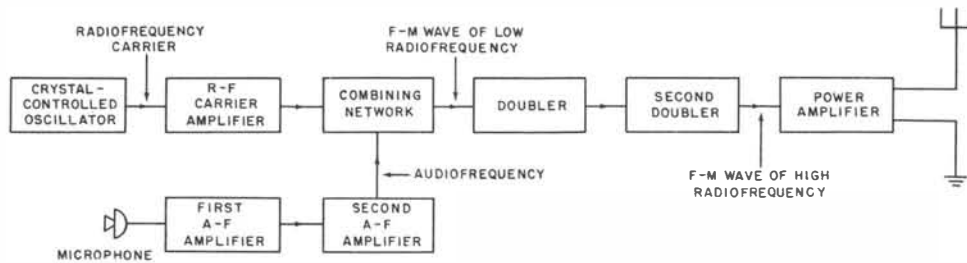
Figure 2-5.—Block diagram of f-m transmitter.
