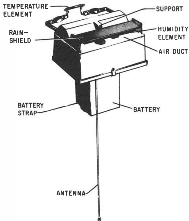
Figure 9-20.—Radiosonde AN/AMT-11( ).
