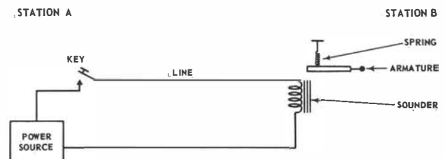
1.196 Figure 4-1.—Manual telegraph circuit.
