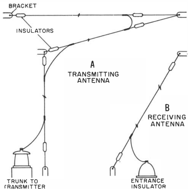
Figure 3-32.—Shipboard wire antennas.
