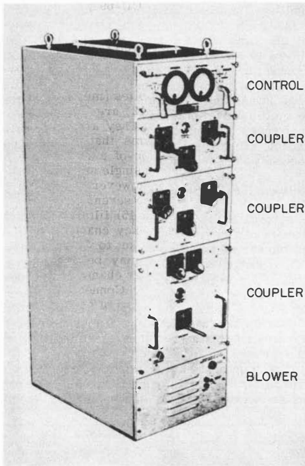
120.12 Figure 3-41.—Antenna multicoupler AN/SRA-23.
