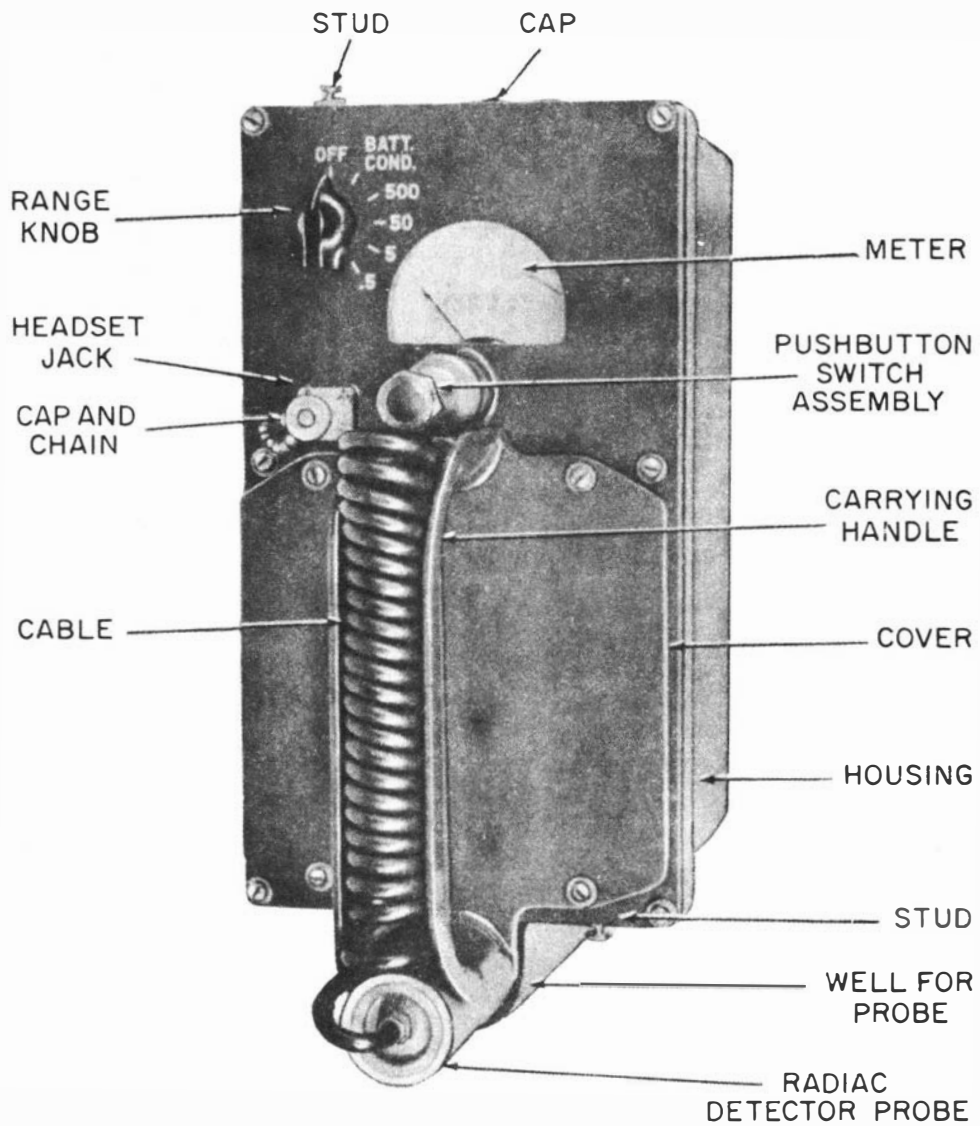
Figure 9-25. —Radiacmeter AN/PDR-27( ).
