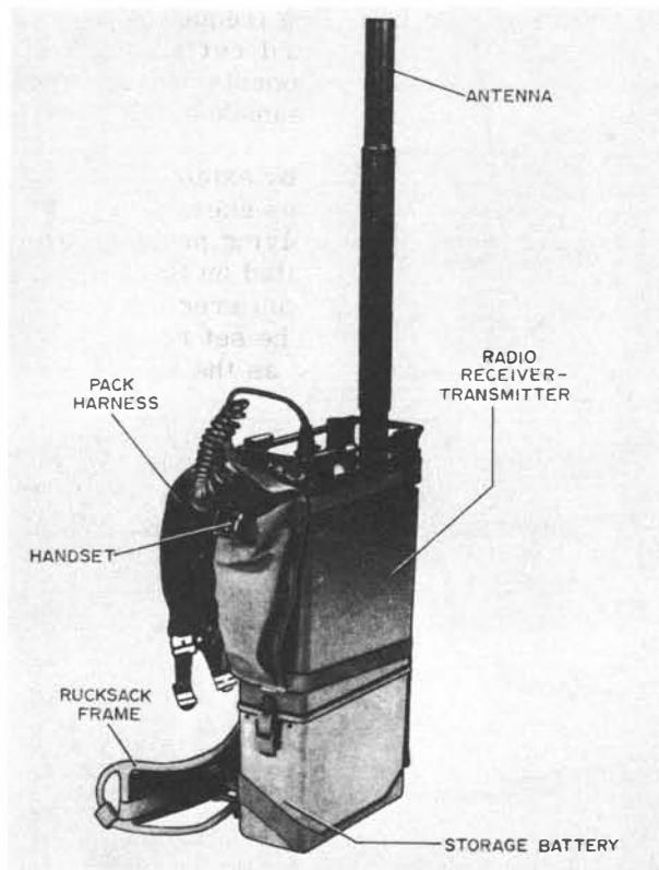
Figure 3-16.—Radio set AN/PRC-41. 120.5
