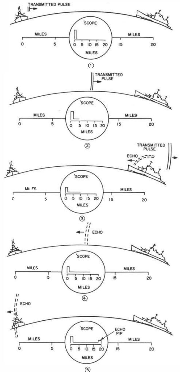
Figure 5-2.—Radar range determination.
