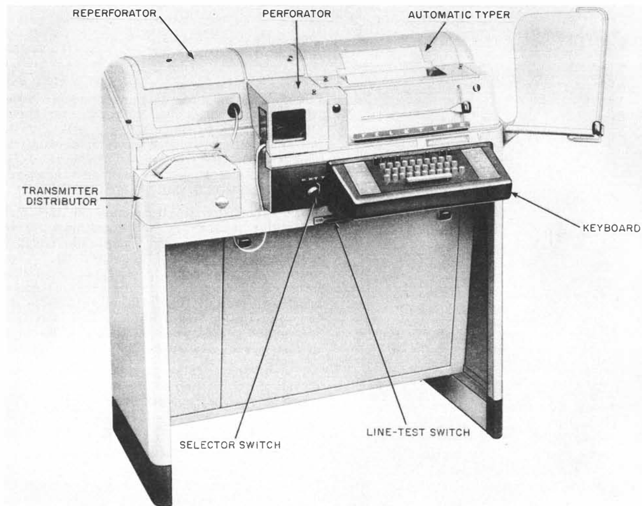
Figure 4-15.—The AN/UGC-6 teletypewriter.
