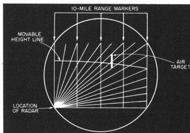
Figure 5-13.—RHI presentation.
