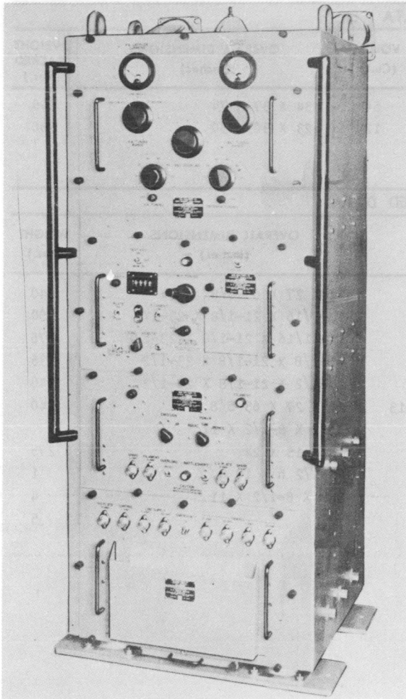
Radio Transmitting Set AN/URT-13
