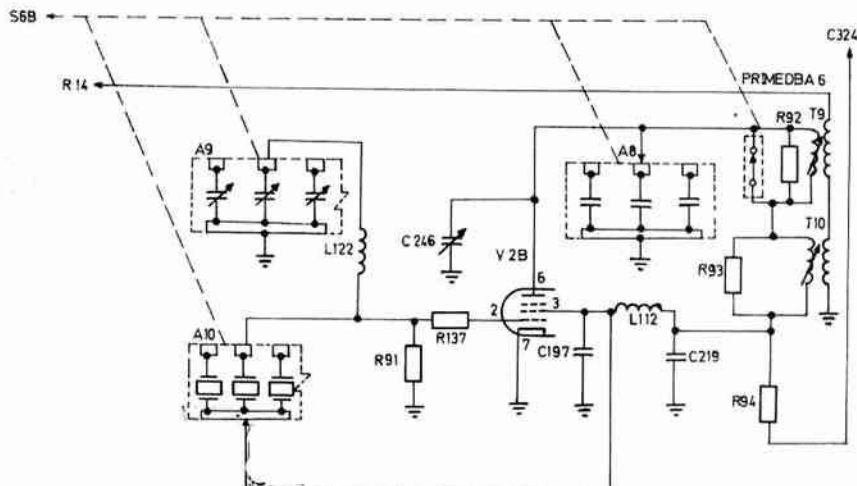
Sl. 21 — Kristal-oscilator
