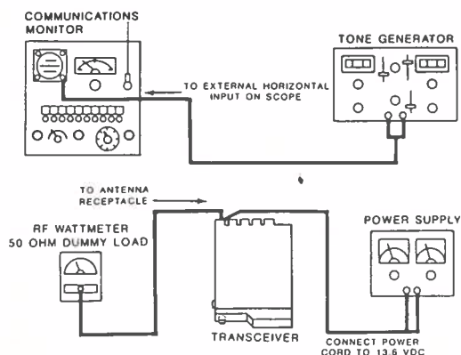
Figure 4. Tone Board Encoder Alignment
