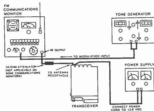
Figure 5. Tone Board Decoder Test
