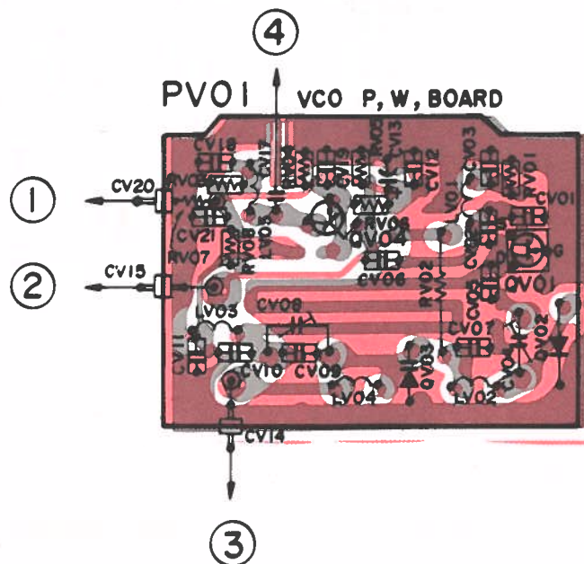
Figure 12. GX3000U Volume, EP-ROM, VCO, and TACT P.C. Boards
