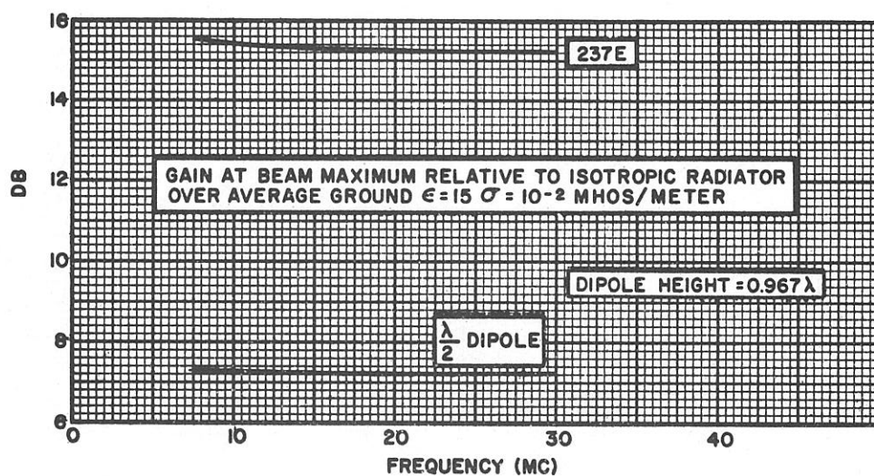
Figure 18. Gain at Beam Maximum Vs Frequency, 237C, D, and E Antennas
