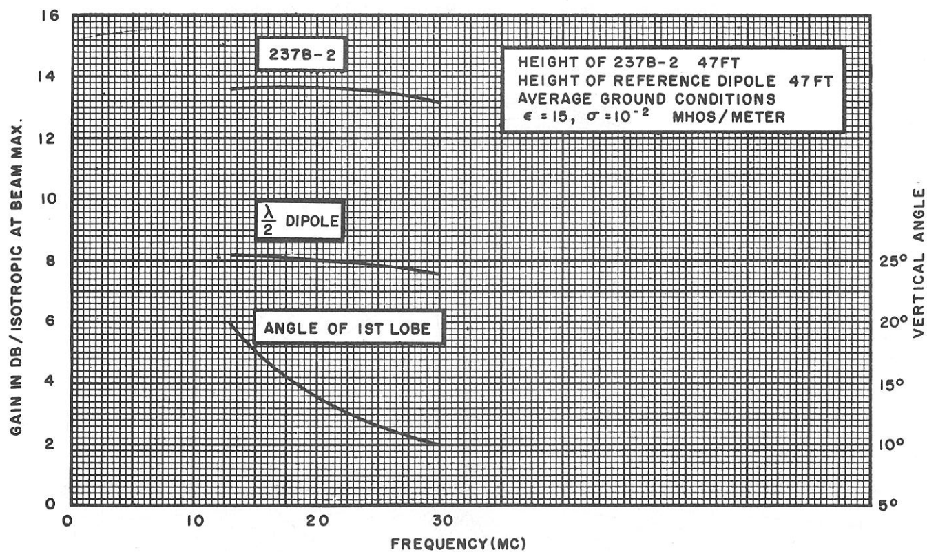
Figure 30. Change in Gain and Vertical Angle of Beam Maximum with Frequency, 237B Antennas
