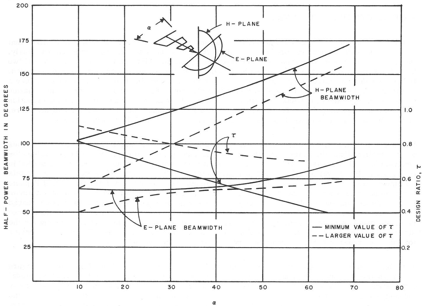
Figure 10. Variation of E- and H-Plane Beamwidths with \alpha for Various Values of Design Ratio
