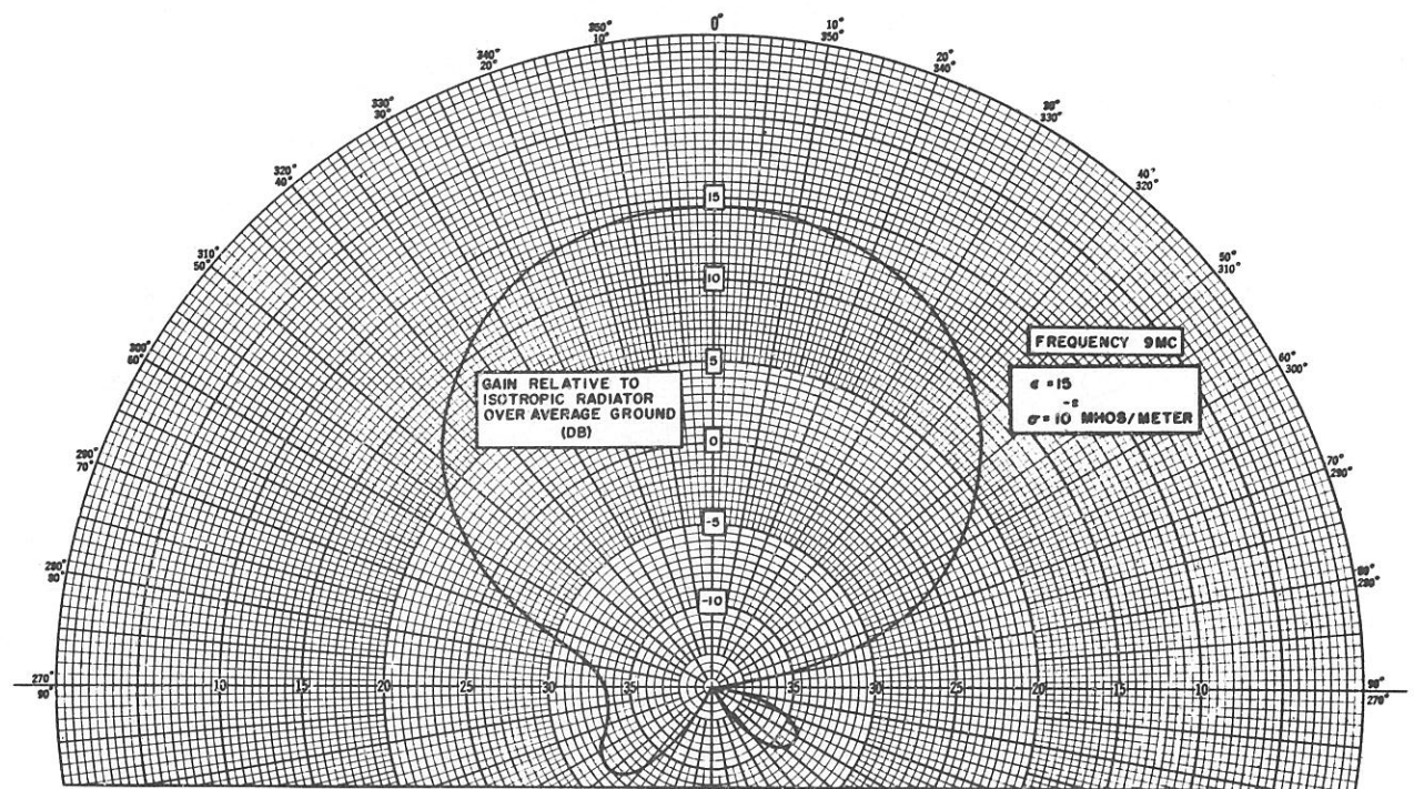
Figure 38A. Azimuth Plane Patterns, 237F-1 Antenna
