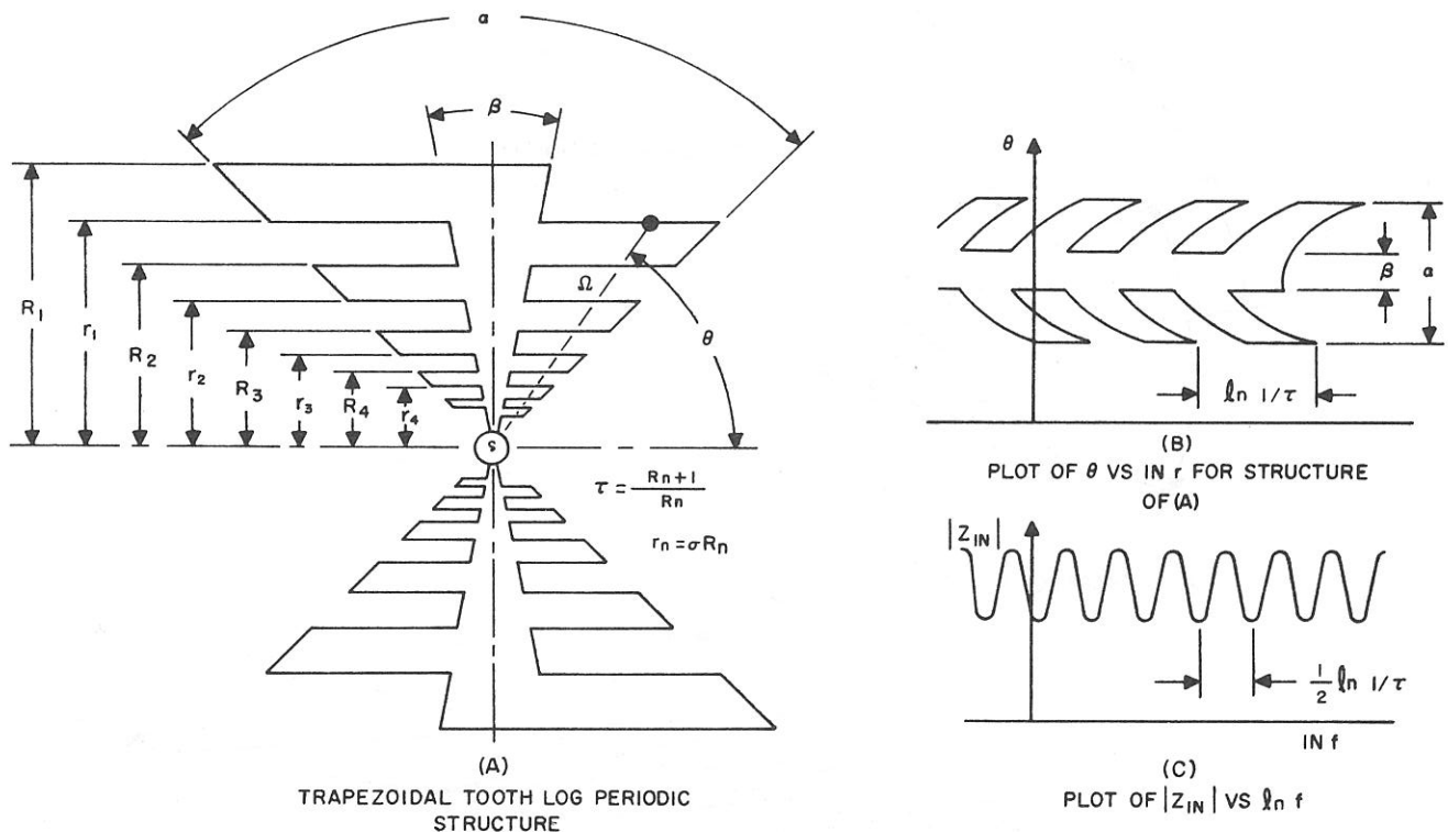
Figure 8. Log-Periodic Antenna Characteristics
