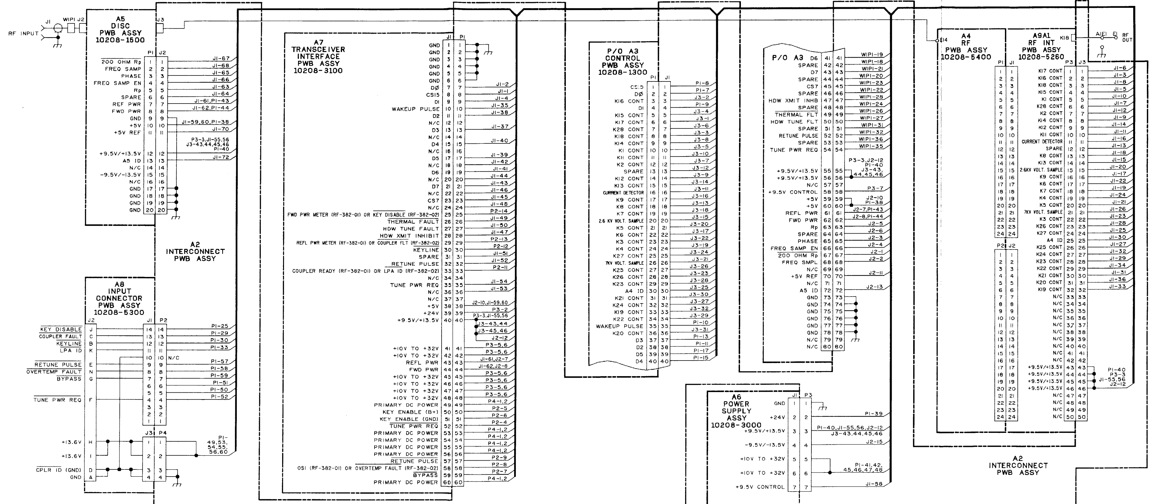
Figure 3. CU-2397/G Antenna Coupler Schematic Diagram (10208-5001, Rev. B)
