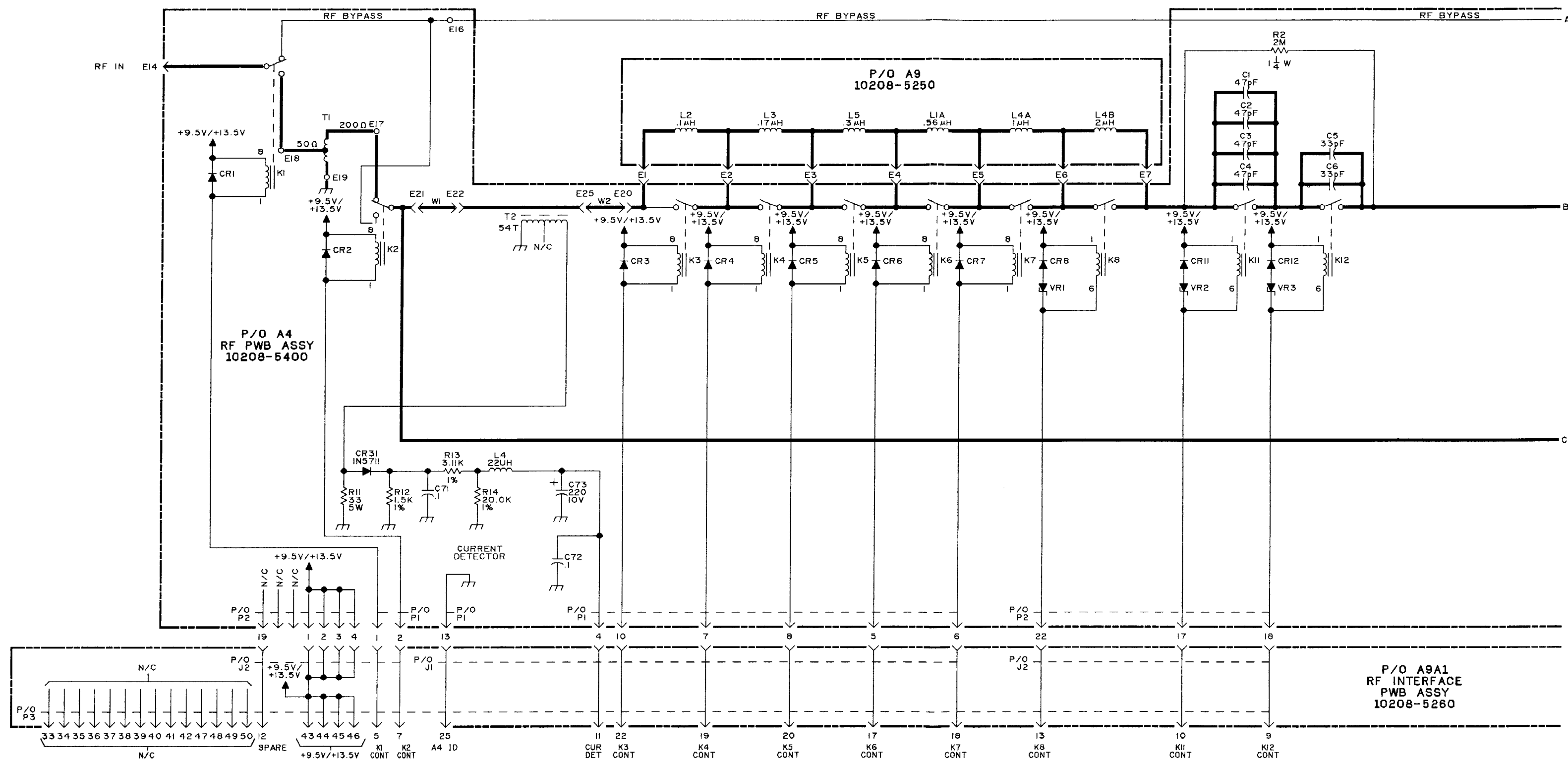
Figure 4. A4 RF PWB Assembly (10208-5400)/ A9 Coil Pack Assembly (10208-5250) Schematic Diagram (10208-5251, Rev. C) (Sheet 1 of 2)
