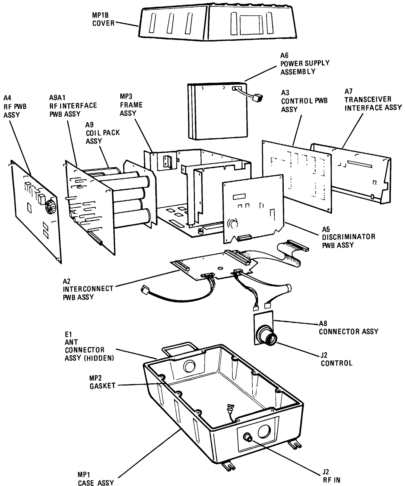
Figure 6-1. Coupler Major Assembly Locations
