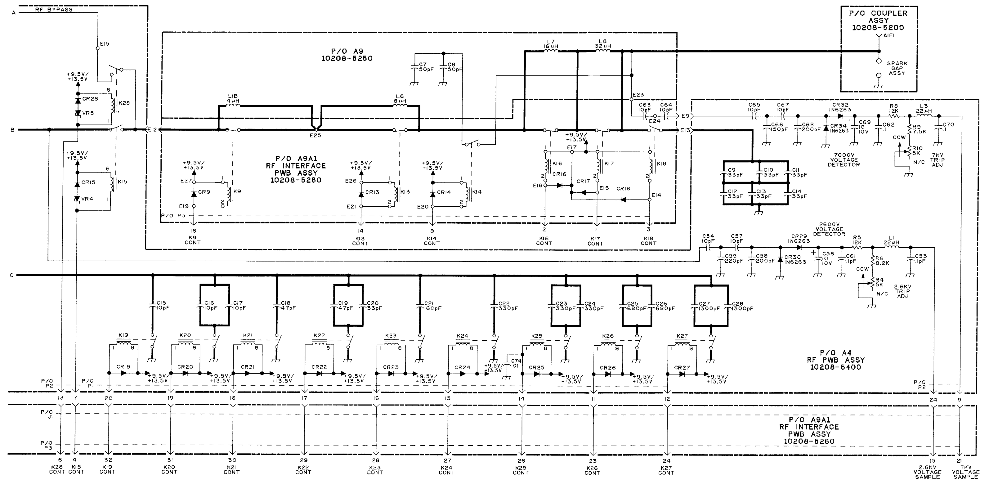
Figure 4. A4 RF PWB Assembly (10208-5400)/ A9 Coil Pack Assembly (10208-5250) Schematic Diagram (10208-5251, Rev. C) (Sheet 2 of 2)
