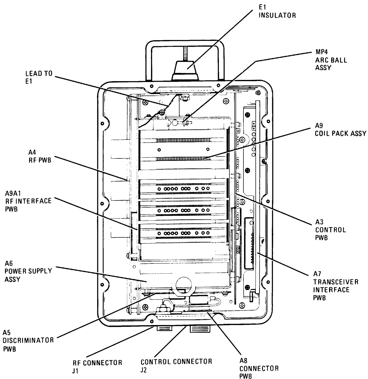
Figure 5-2. Coupler Major Assemblies
