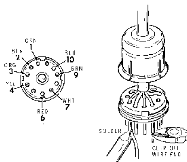
Detail 7F
