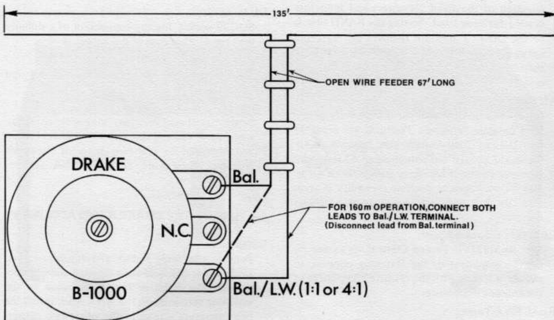
Figure 3 Multiband Antenna
