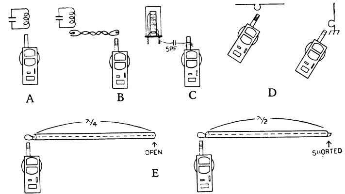
Fig. 1 Dip meter coupling methods.
