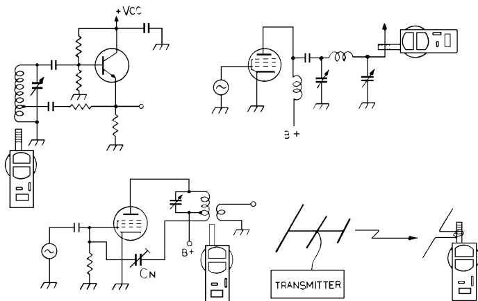
Fig. 2 Absorption wavemeter applications.
