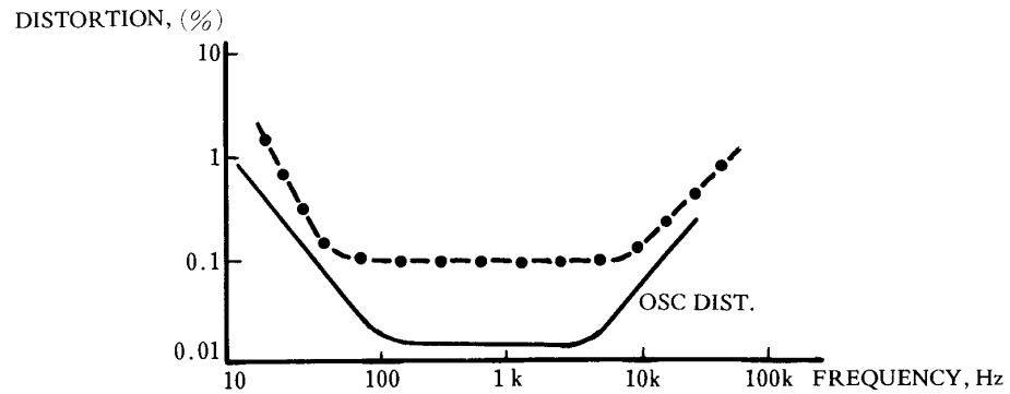
Fig. 2-9 B : Frequency VS. distortion.
