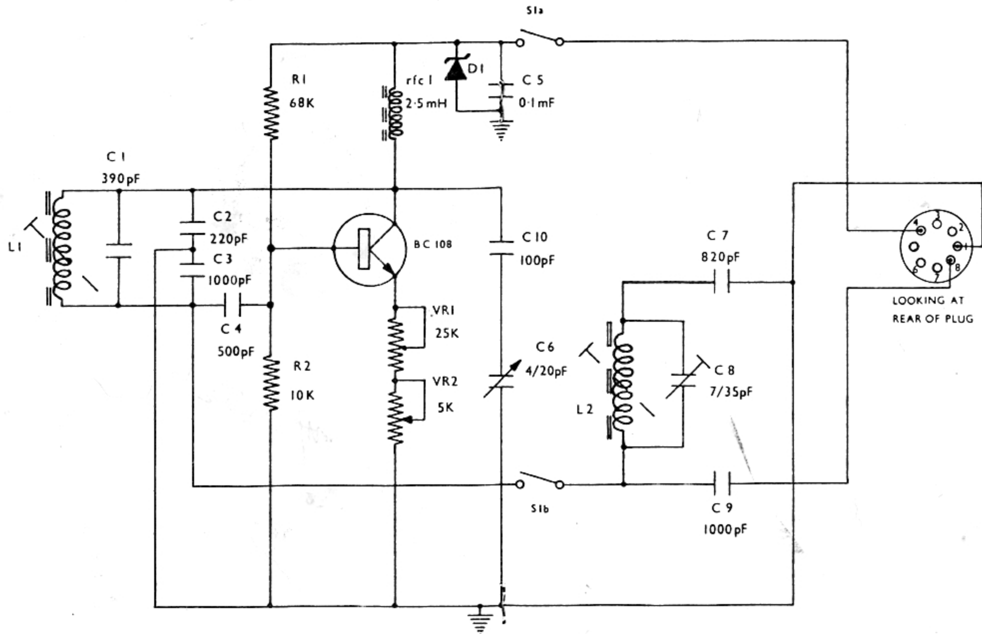
KW 110 Circuit Diagram
