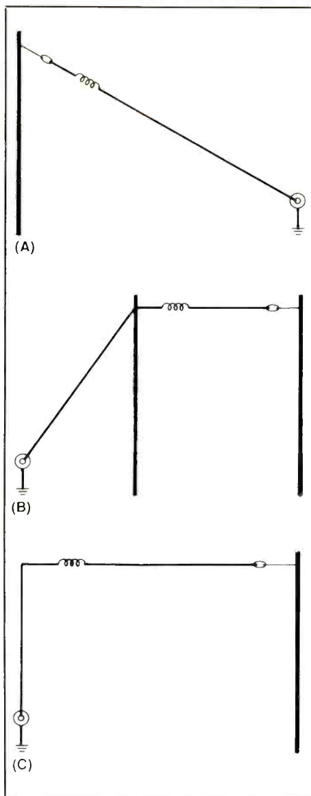
Fig. 5. Various configurations for duo-banders.
