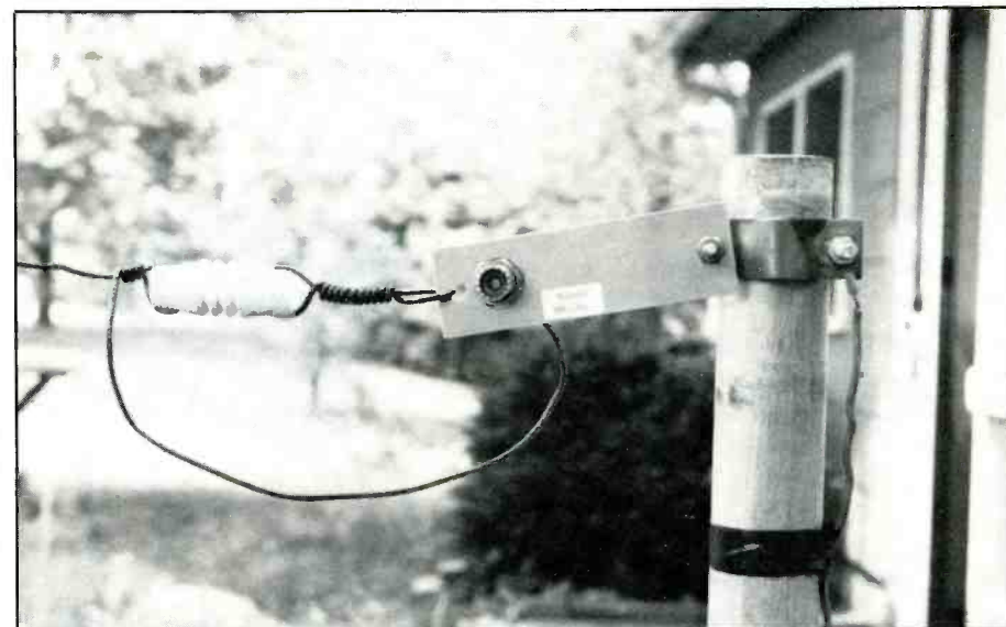
Fig. 3. Ground level feeding of duo-bander. A short length of cable connects antenna to transceiver.
