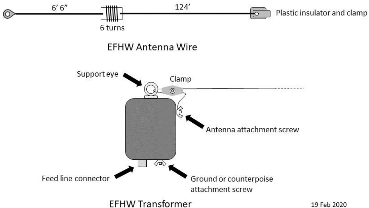
Figure 1 – EFHW Transformer Unit and Antenna Wire
