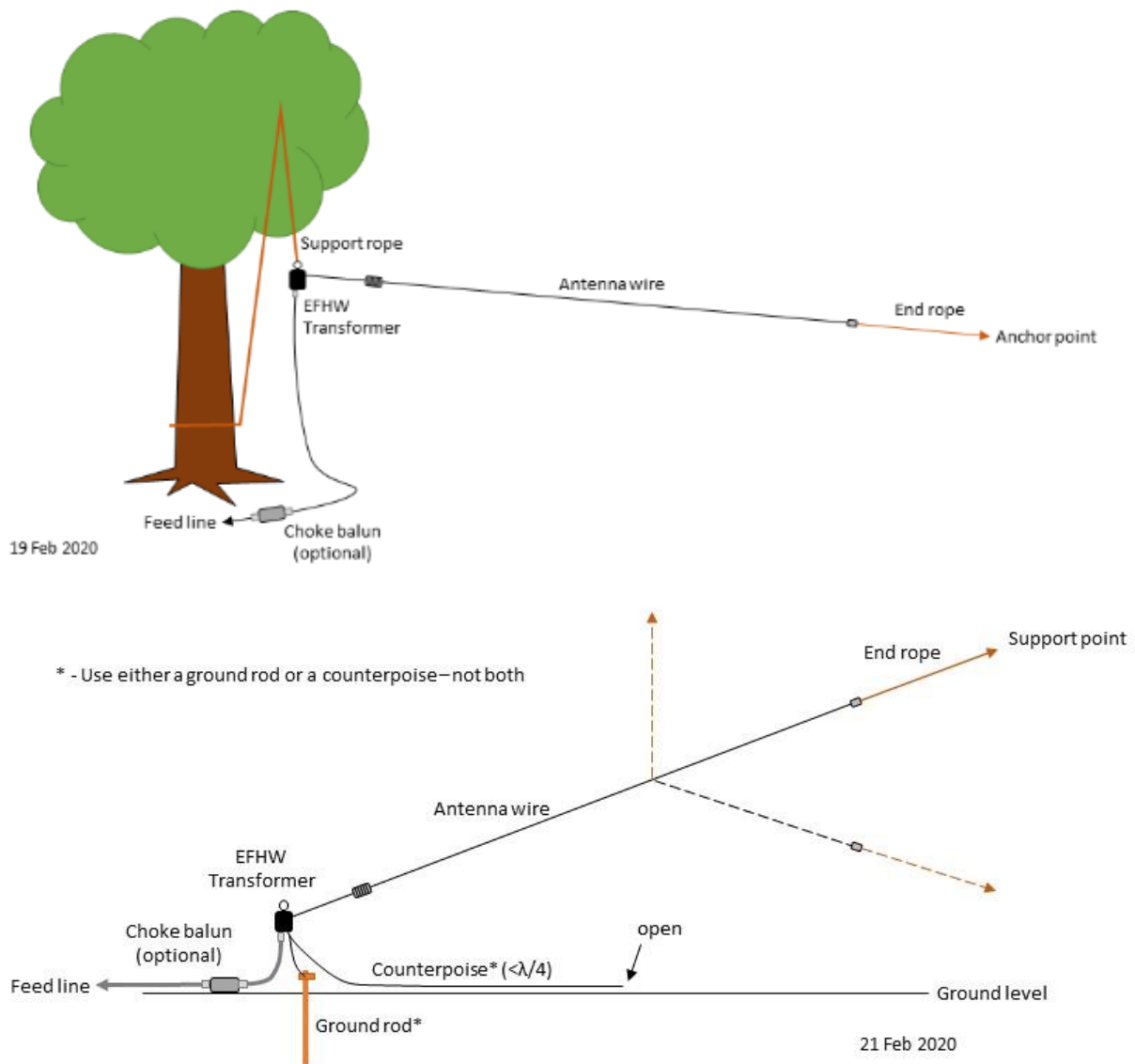
Figure 2A (top) and 2B (bottom) – Typical EFHW Installations
