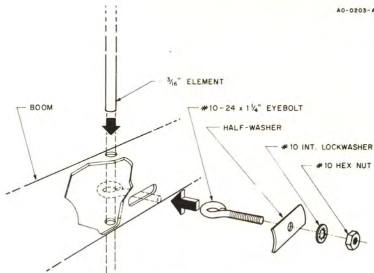
DETAIL A
