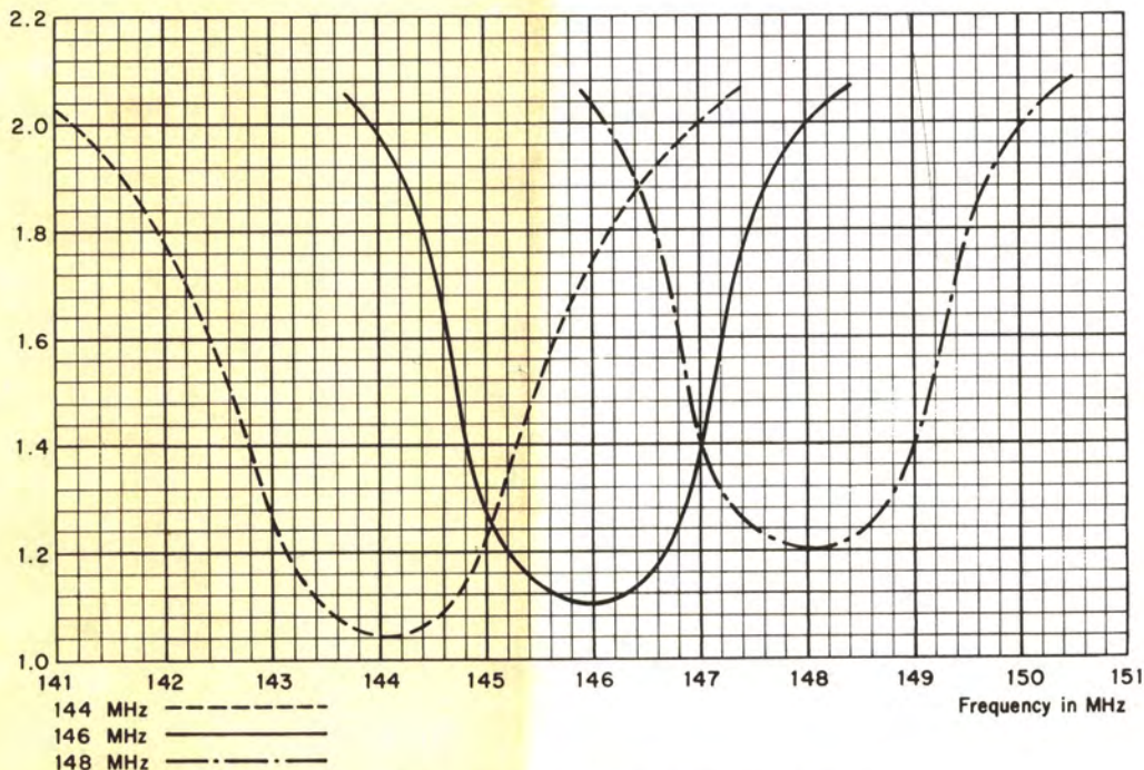
VSWR for Horizontal Polarization Only
