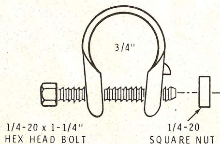
ELEMENT CLAMPS
