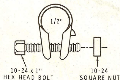
ELEMENT CLAMPS
