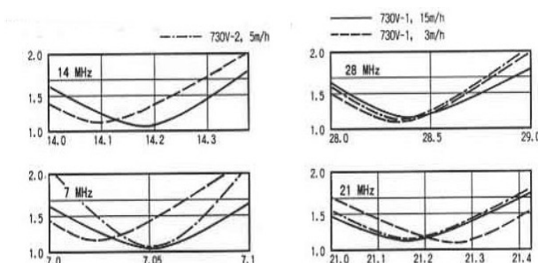
Figure 2. VSWR Characteristic 730V-1, 730V-2, (730V-xA/HF) V Angle: 90°
