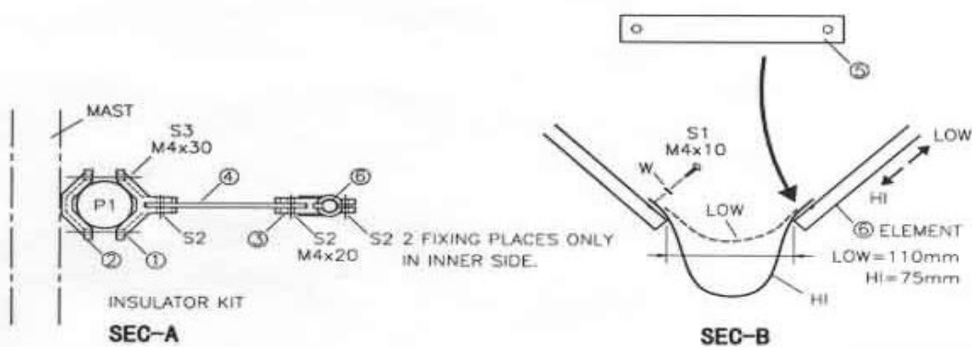
FIGURE 6. 50MHZ RADIATOR ELEMENT ASSEMBLY/730V-xA. CMN9710 DWA.0068
