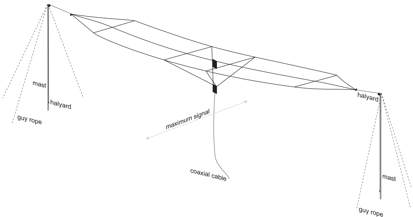
Figure 6: Horizontal configuration
