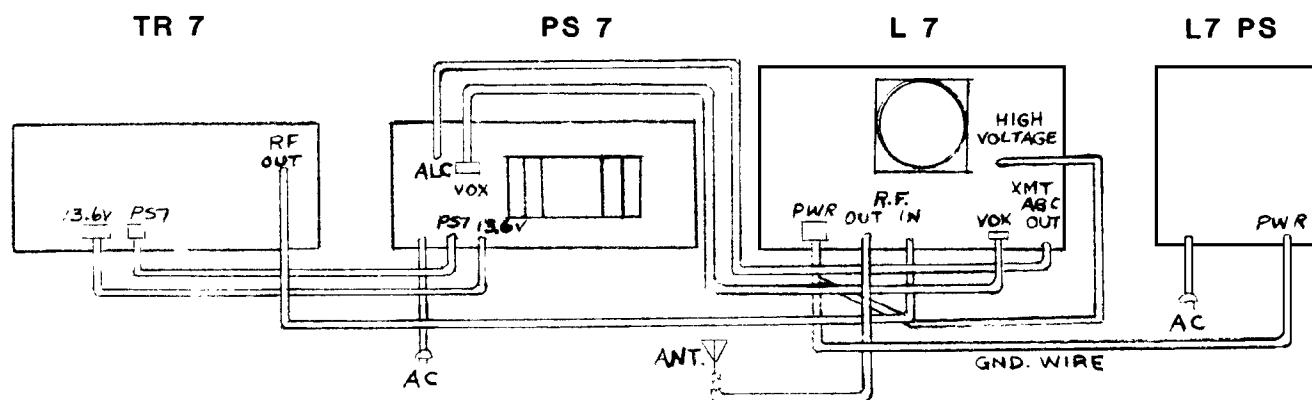
Fig. 2-4 Connecting the PS-7 Power Supply and the R. L. Drake Line of Compatible Exciters
