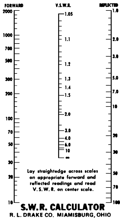
Figure 3-3. SWR Nomograph
