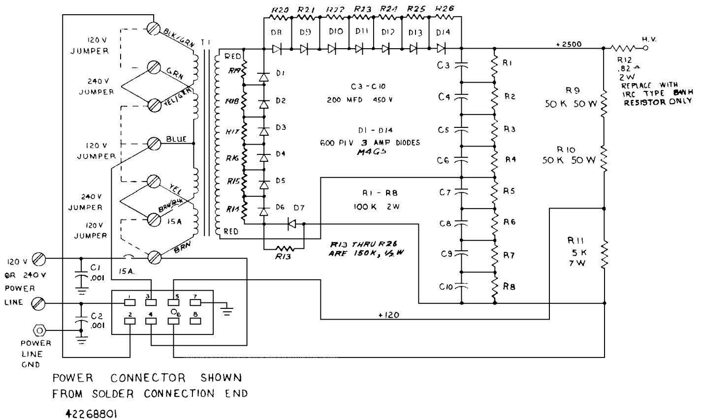
Fig. 5-4 Model L7 Power Supply Schematic Diagram
