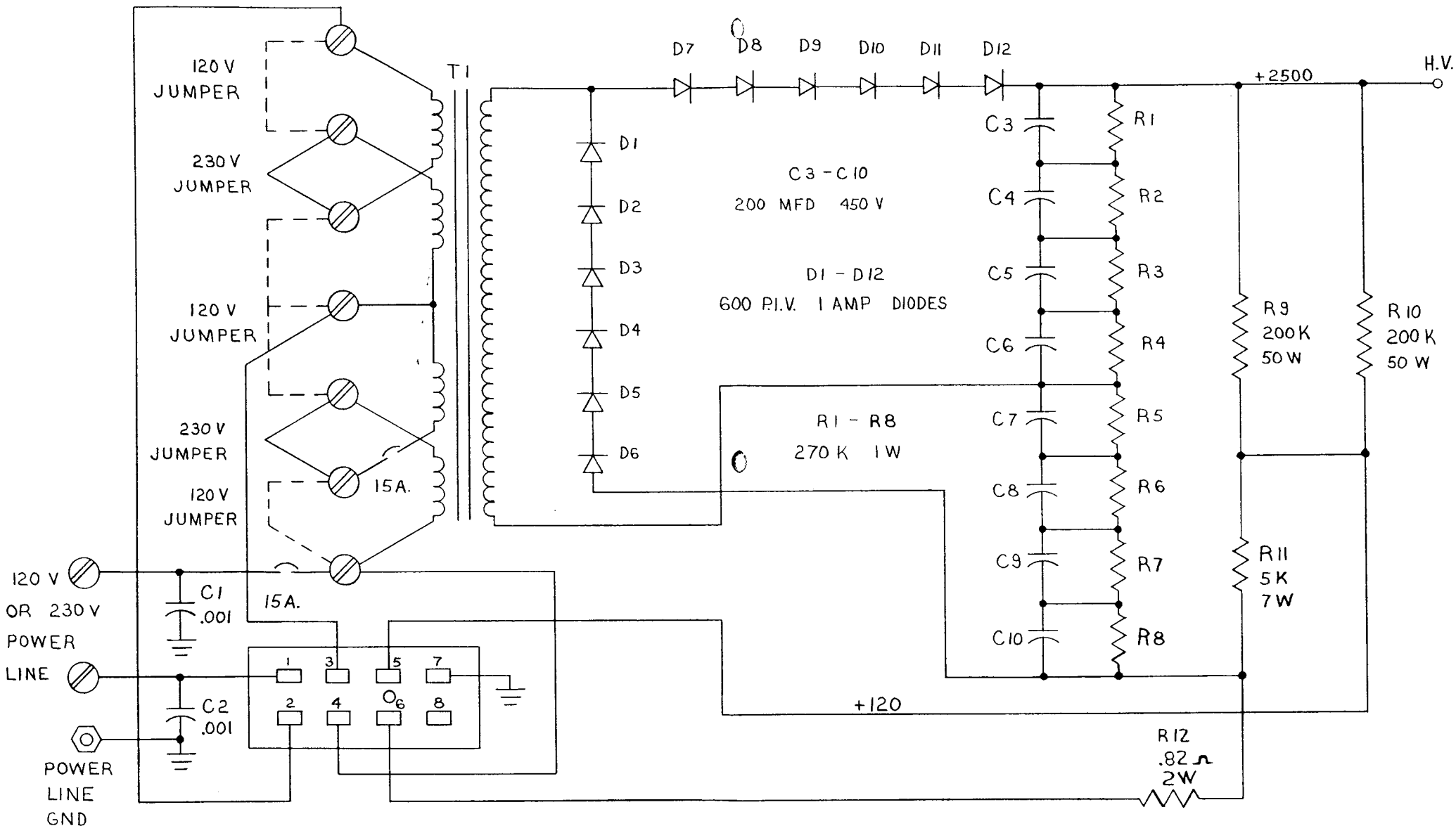
SCHEMATIC DIAGRAM MODEL L-4 PS POWER SUPPLY
