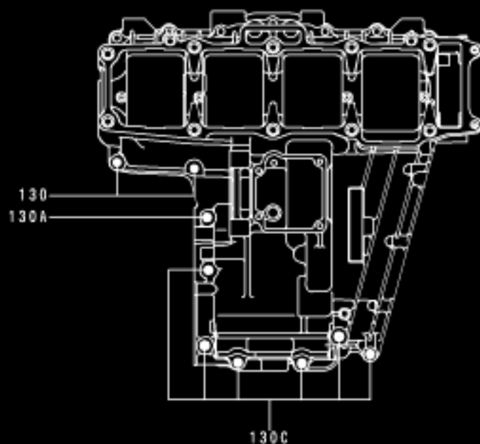
Crankcase Lower
