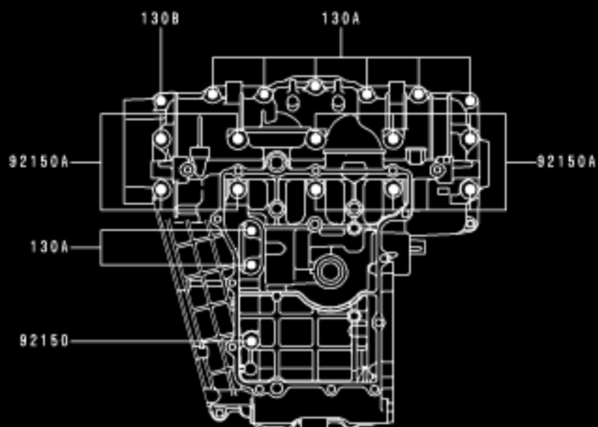
Crankcase Lower
