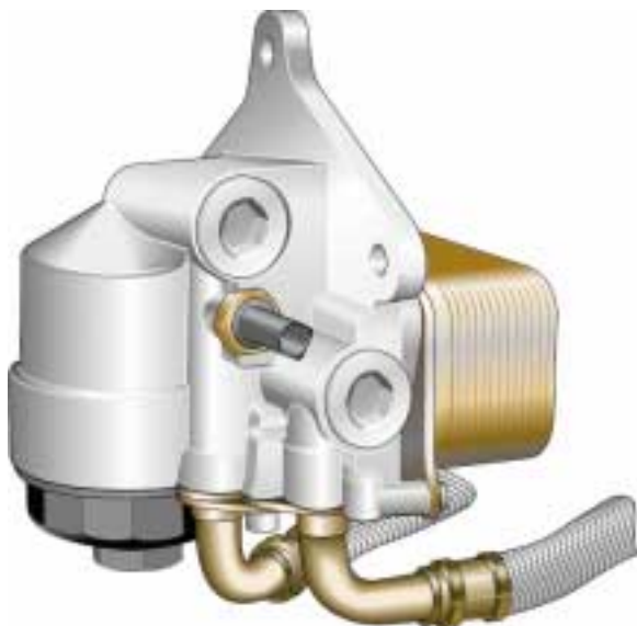
Oil filter/cooler module of the W8
