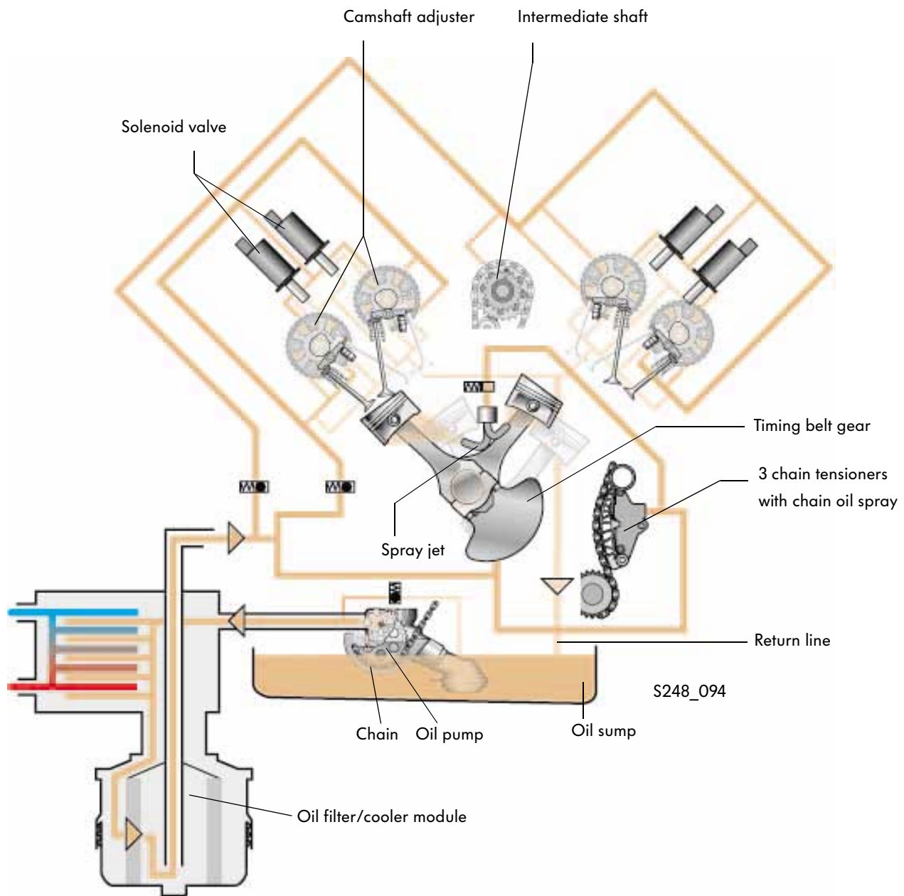
Oil sump of the W8 engine
