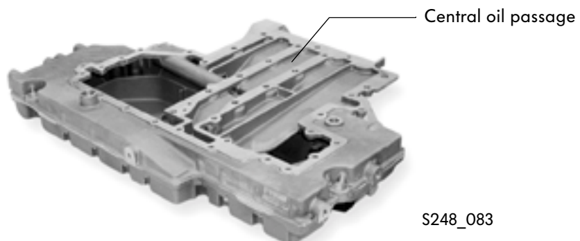
Oil sump of the W8 engine
