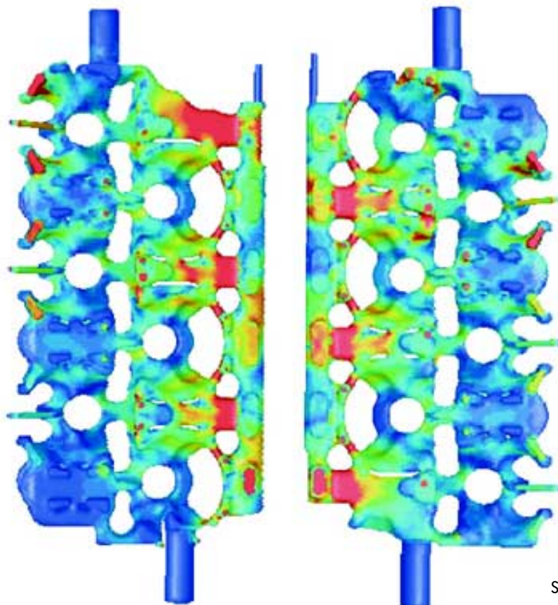
Coolant flows into the cylinder heads
