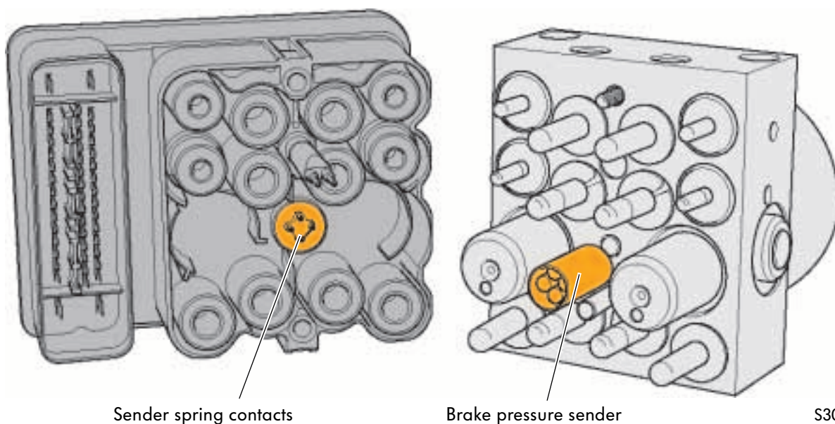
Hydraulic unit with brake pressure sender
