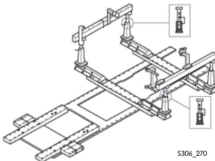
Portal gauge supplement VAS 5007/17
