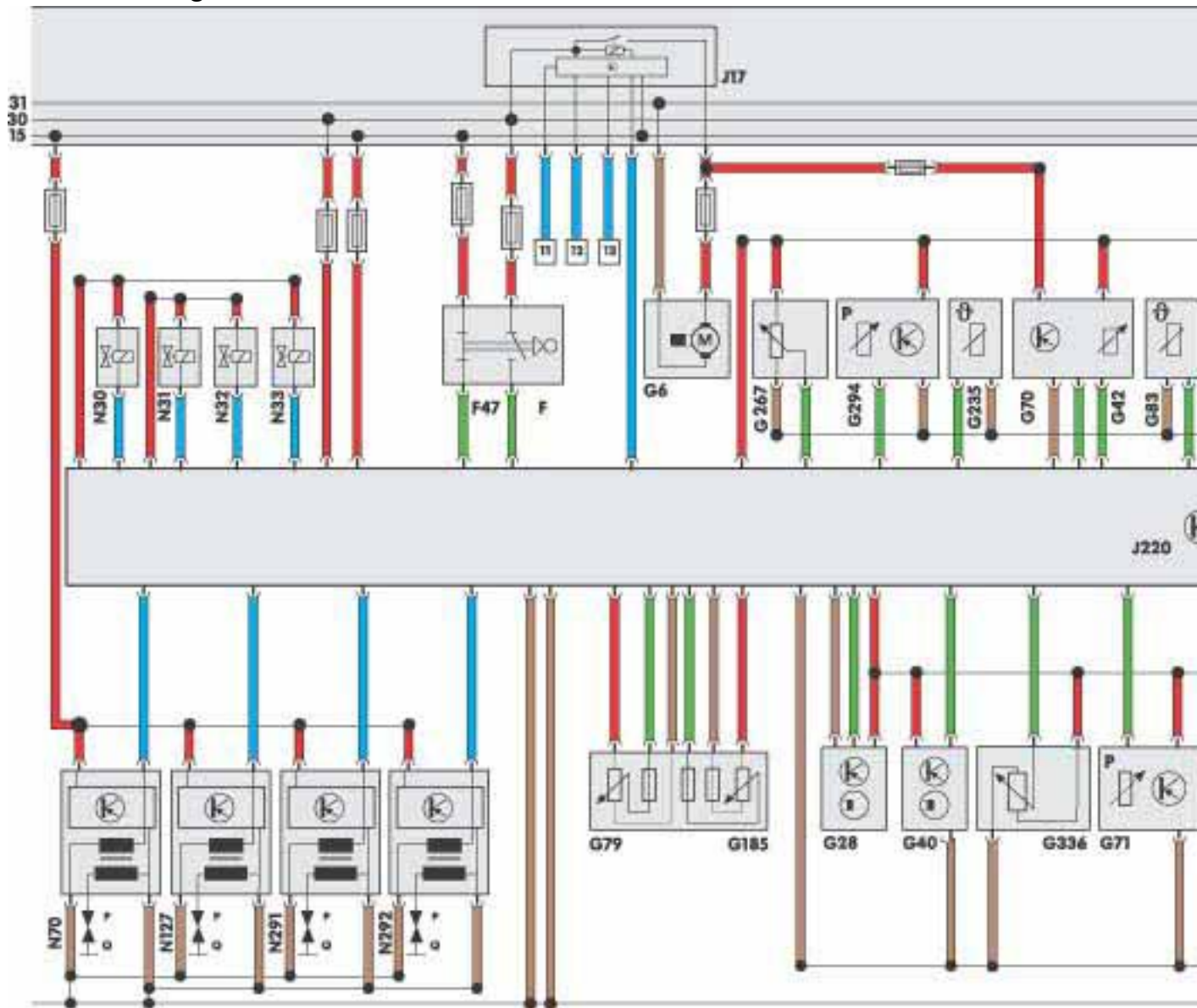
Function diagram
