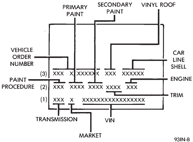
Fig. 2 Body Code Plate Decoding BODY CODE PLATE—LINE 3
