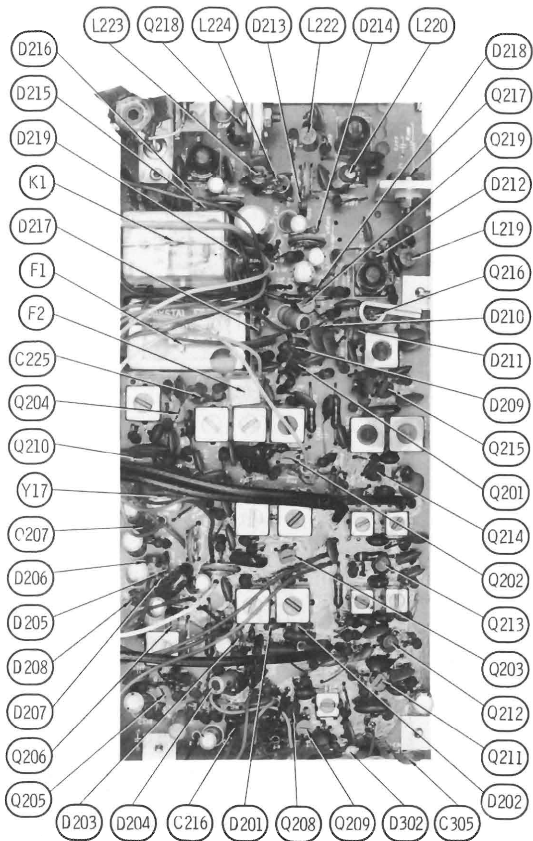
200 SERIES COMPONENT BOARD
