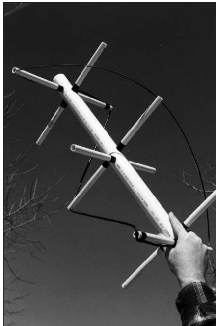
Fig 55 — The antenna with two of the four legs in place. The ends of the PVC cross arms that hold the coaxial leg are notched; the wire elements pass through holes drilled in the ends of their supporting cross arms.
