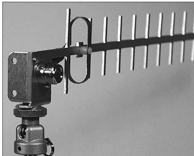
Fig 21 — Directional antennas, such as this MFJ 2.4 GHz Yagi, are best for HSMM links.
