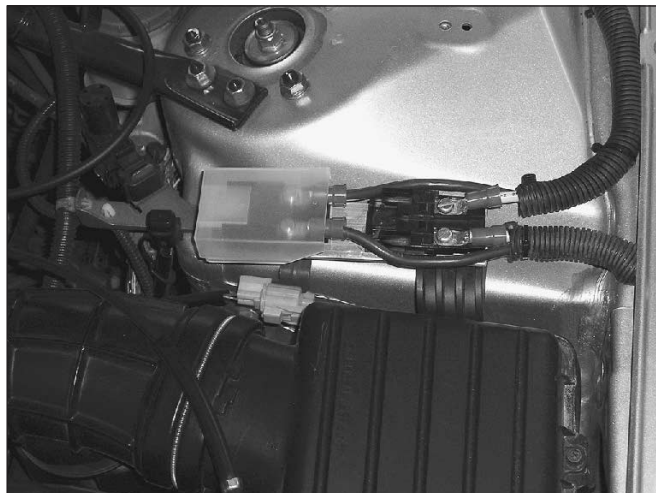
Fig 29.21 — Wiring attached to a fuse block.
