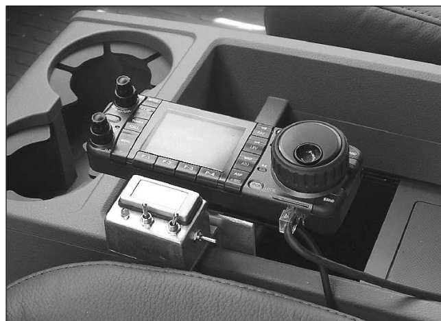
Fig 29.17 — In this mobile installation, the transceiver control head is mounted in the center console, next to a box with switches for adjusting the antenna.
