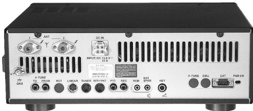
Fig 29.10 — The back of this Yaesu FT-950 transceiver shows some of the many types of connectors encountered in the amateur station. Note that this variety is found on a single piece of equipment.
