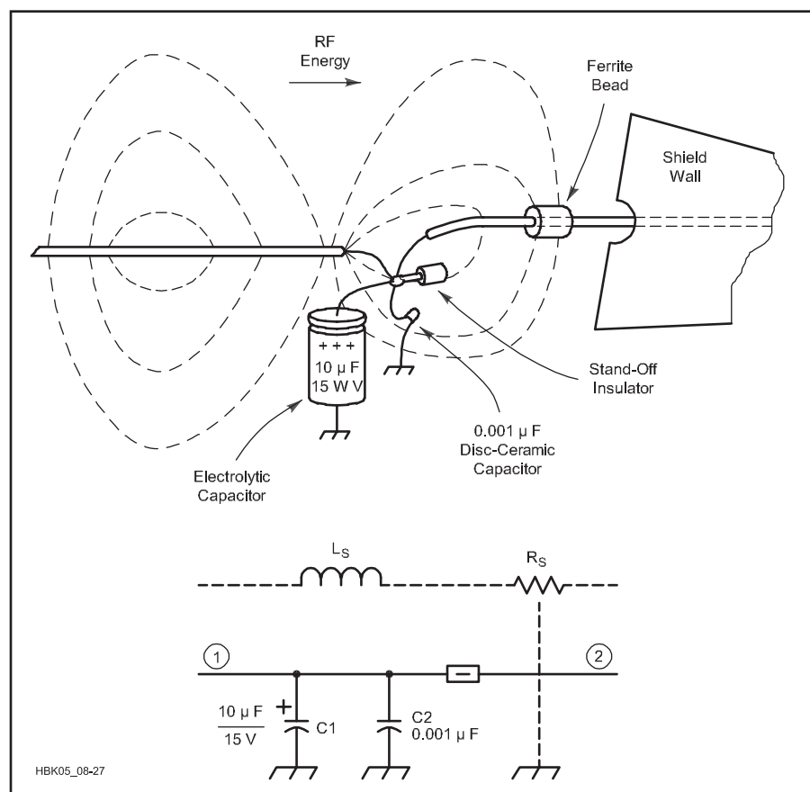
Fig 23.24 — Two capacitors in parallel afford better bypassing across a wide frequency range.
