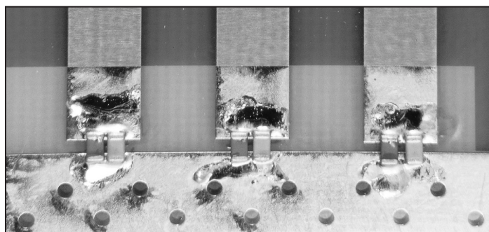
Fig 23.30 — Printed comb-line filter uses two chip capacitors in parallel to reduce loss.
