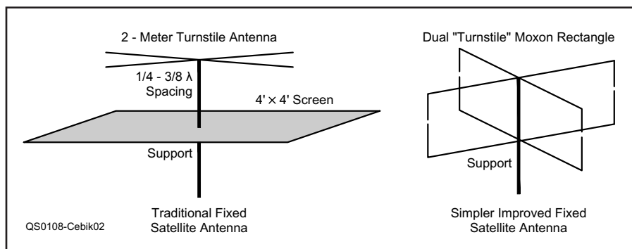
Fig 21.112 — Alternative schemes for fixed-position satellite antennas: the traditional turnstile-and-screen and a pair of “turnstile” Moxon rectangles.
