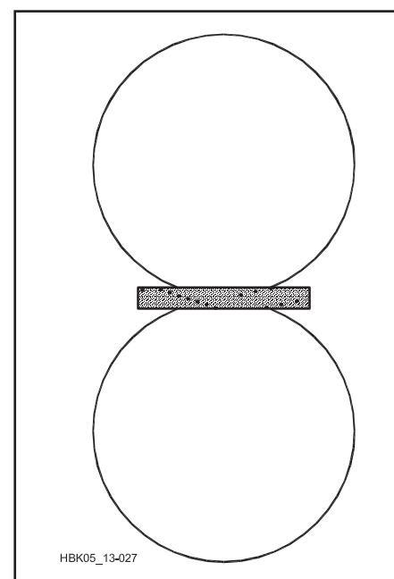
Fig 21.117 — Field pattern for a ferrite-rod antenna. The dark bar represents the rod on which the loop turns are wound.
