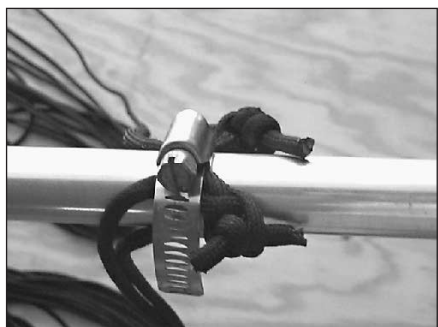
Fig 21.56 — Guys are made of Dacron line that is attached to the HVD by a stainless-steel worm-screw-type hose clamp. A self-tapping sheet-metal screw (not visible in the photo) prevents the clamp from sliding down the antenna.
