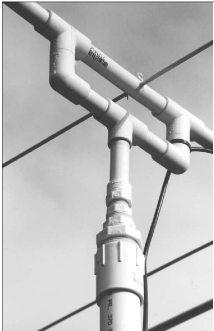
Fig 21.105 — The completed 2 meter Yagi is shown with the PVC boom and mast mount.
