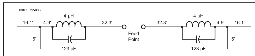
Fig 21.34 — A W8NX multiband dipole for 80, 40, 20, 15 and 10 meters. The values shown (123 pF and 4 \mu H) for the coaxial-cable traps are for parallel resonance at 7.15 MHz. The low-impedance output of each trap is used for this antenna.
