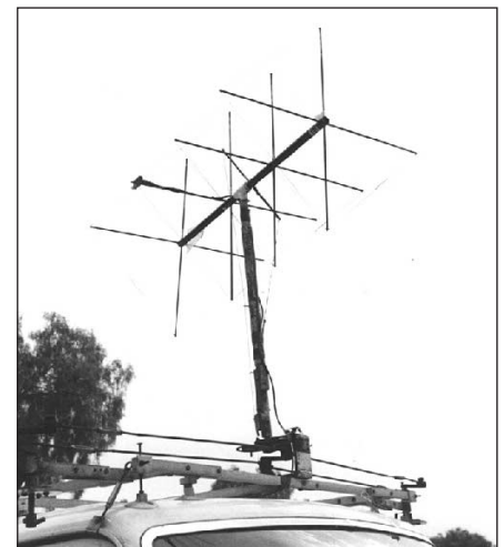
Fig 21.123 — The mobile RDF installation of WB6ADC features a thin wire quad that can be switched between vertical and horizontal polarization.
