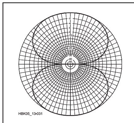
Fig 21.121 — The pattern of an Adcock array with element spacing of \frac{1}{2} wavelength. The elements are aligned with the vertical axis.
