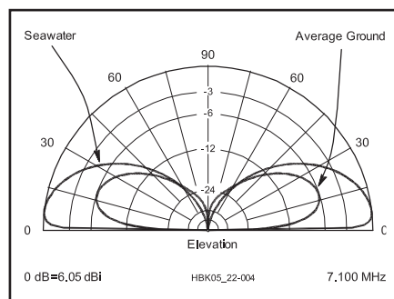
Fig 21.8 — Elevation patterns for a vertical dipole over sea water compared to average ground. In each case the center of the dipole is just over \frac{1}{4}\lambda high. The low-angle response is greatly degraded over average ground compared to sea water, which is virtually a perfect ground.
