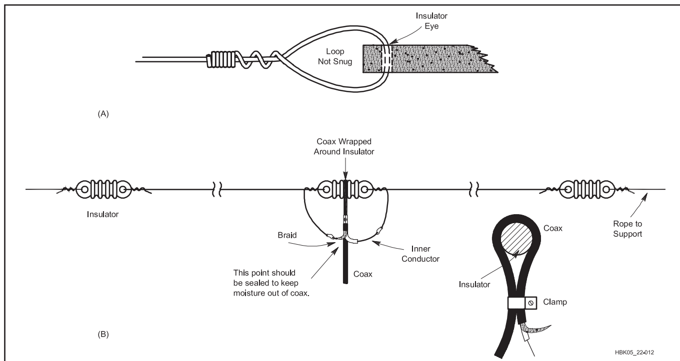
Fig 21.16 — Details of dipole antenna construction. The end insulator connection is shown at A, while B illustrates the completed antenna. This is a balanced antenna and is often fed with a balun at the feed point as described in the text.
