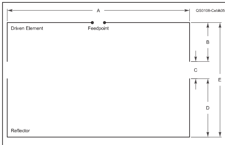
Figure 21.114 — The basic dimensions of a Moxon rectangle. Two identical rectangles are required for each “turnstiled” pair. See Table 21.27 for letter references.
