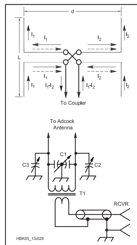
Fig 21.119 — A simple Adcock antenna and its coupler.
