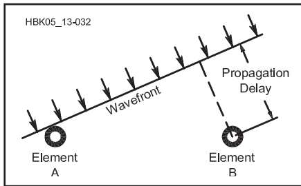
Fig 21.122 — One technique used in electronic beam forming. By delaying the signal from element A by an amount equal to the propagation delay, two signals are summed precisely in phase, even though the signal is not in the broadside direction.
