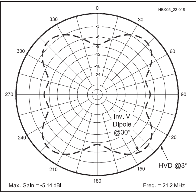
Fig 21.21 — Azimuth patterns at 3^\circ elevation for the HVD (solid line) and inverted-V (dashed line).
