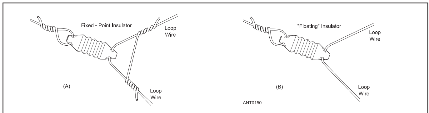
Fig 21.78 — Two methods of installing the insulators at the loop corners.
