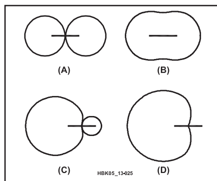
Fig 21.115 — Small loop field patterns with varying amounts of antenna effect — the undesired response of a loop acting merely as a mass of metal connected to the receiver antenna terminals. The horizontal lines show the plane of the loop turns.
