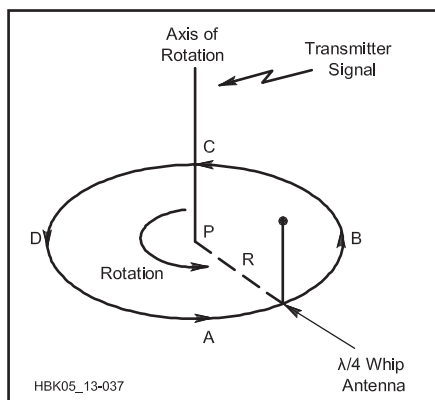
Fig 21.126 — A theoretical Doppler antenna circles around point P, continuously moving toward and away from the source at an audio rate.
