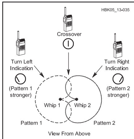
Fig 21.124 — In a switched pattern RDF set, the responses of two cardioid antenna patterns are summed to drive a zero center indicator.
