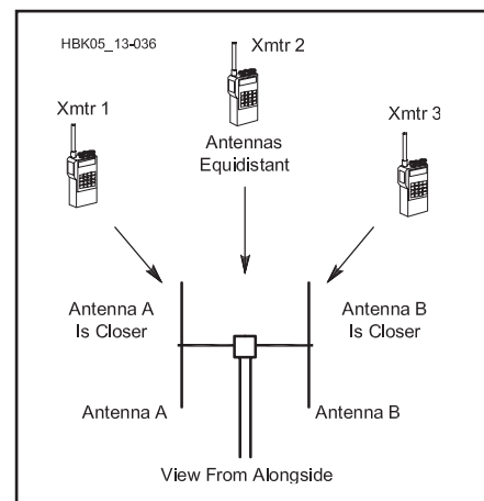
Fig 21.125 — A dual-antenna TDOA RDF system has a similar indicator to a switched pattern unit, but it obtains bearings by determining which of its antennas is closer to the transmitter.
