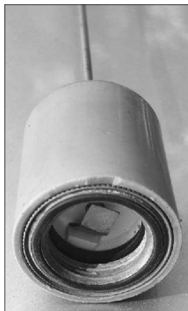
Fig 21.93 — The NMO (New Motorola) mount is widely used for VHF and UHF mobile antennas. It is available in mag-mount, trunk and lip mount and through-body mounting styles.
