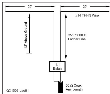
Fig 21.42 — Basic configuration of the triband dipole, consisting of a 58-foot doublet fed with 35.5 feet of 600 \Omega open-wire feed line. SWR at the balun input is approximately 1.5:1 on 17 meters and 2.4:1 on 12 meters and 30 meters.
