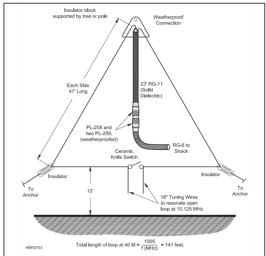
Fig 21.76 — NT4B's 30 and 40 meter loop is fed at the top via a quarter-wave 40 meter matching transformer made of 75 \Omega coax. Note the 18 inch tuning wires used to lower the antenna's 30 meter resonance from 10.5 to 10.1 MHz. Adjust the length of these wires to set the 30 meter resonant frequency.
