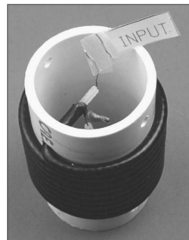
Fig 21.38 — Other views of a W8NX coax-cable trap.
