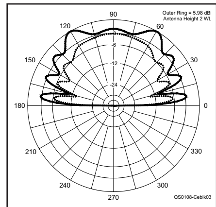
Fig 21.113 — A comparison of elevation patterns for the turnstile-and-screen system (with \frac{3}{8}\lambda wavelength spacing, shown by the solid black line) and a Moxon pair (dashed line), both at 2 λ height.
