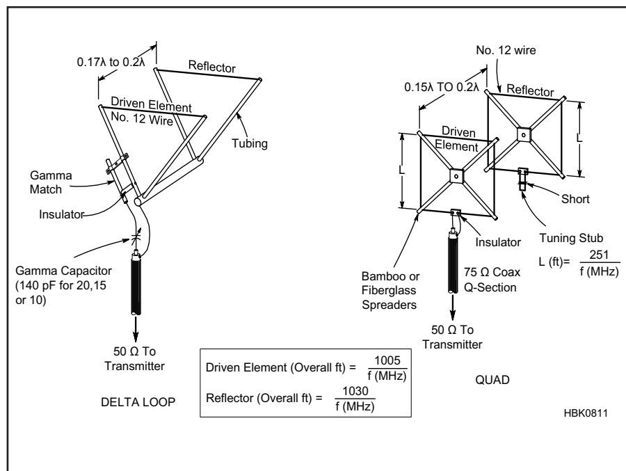
Fig 21.71 — Information on building a quad or a delta-loop antenna. The antennas are electrically similar, but the delta-loop uses plumber's delight construction. The \lambda/4 length of 75 \Omega coax or Q-section acts as a synchronous transmission-line transformer from the approximate 100 \Omega feed point impedance of the quad to the 50 \Omega feed line.
