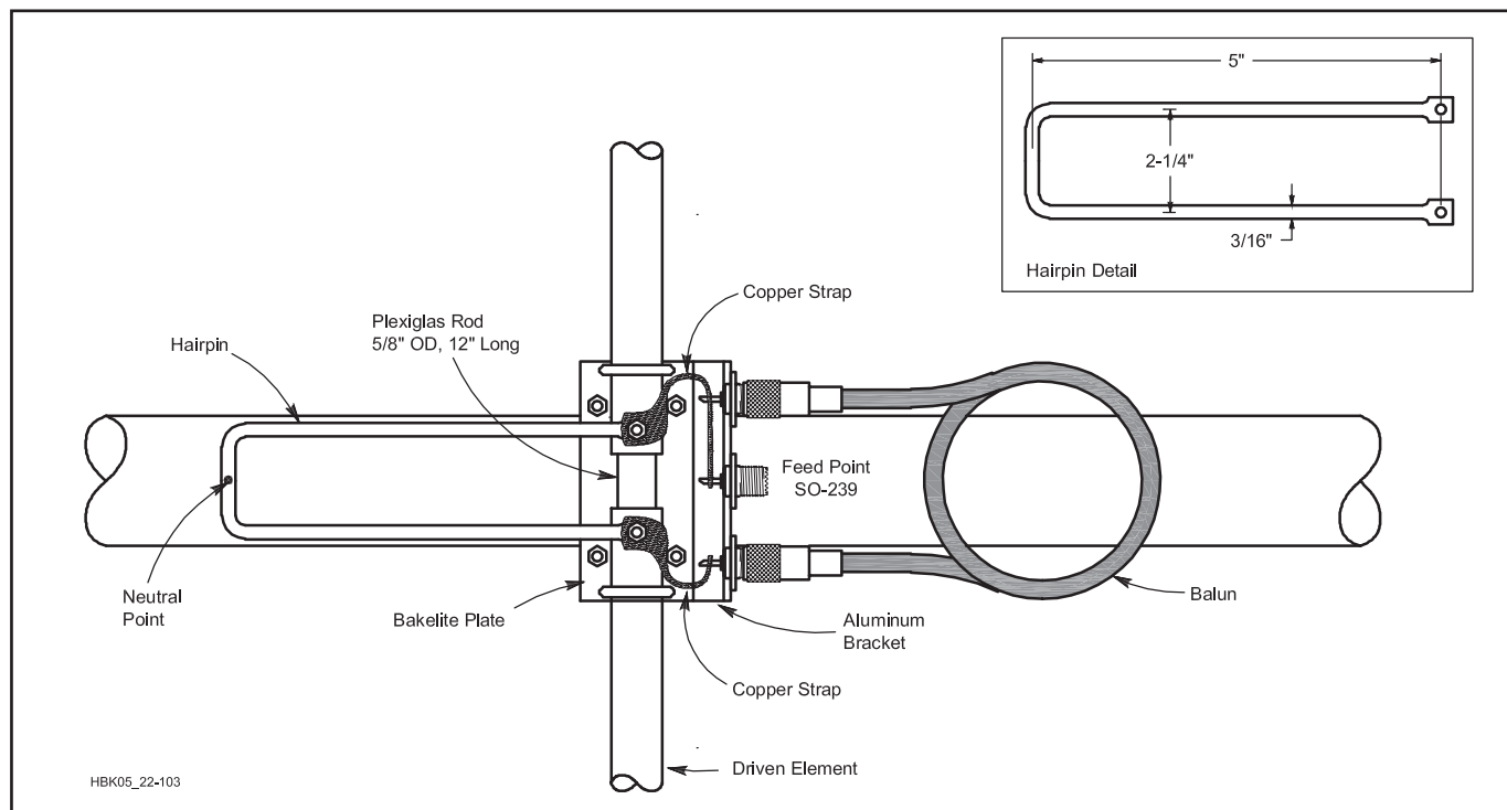
Fig 21.104 — Detailed drawing of the feed system used with the 50 MHz Yagi. Balun lengths: For cable with 0.80 velocity factor — 7 feet, 10 \frac{3}{4} inches. For cable with 0.66 velocity factor — 6 feet, 5 \frac{3}{4} inches
