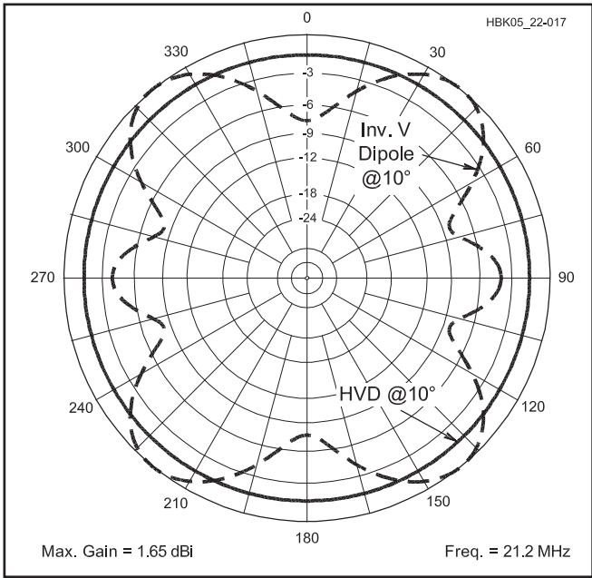
Fig 21.20 — Azimuth patterns at 10^\circ elevation for the HVD (solid line) and inverted-V (dashed line).
