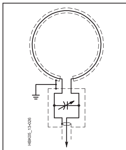
Fig 21.116 — Electrostatically-shielded loop for RDF. To prevent shielding of the loop from magnetic fields, leave the shield unconnected at one end.
