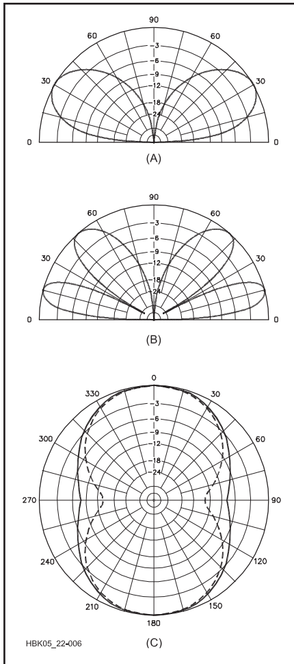
Fig 21.10 — At A, the elevation response pattern of a dipole antenna placed \frac{1}{2}\lambda above a perfectly conducting ground. At B, the pattern for the same antenna when raised to 1\lambda . For both A and B, the conductor is coming out of the paper at a right angle. C shows the azimuth patterns of the dipole for the two heights at the most-favored elevation angle, the solid-line plot for the \frac{1}{2}\lambda height at an elevation angle of 30^\circ , and the broken-line plot for the 1\lambda height at an elevation angle of 15^\circ . The conductor in C lies along the 90^\circ to 270^\circ axis.
