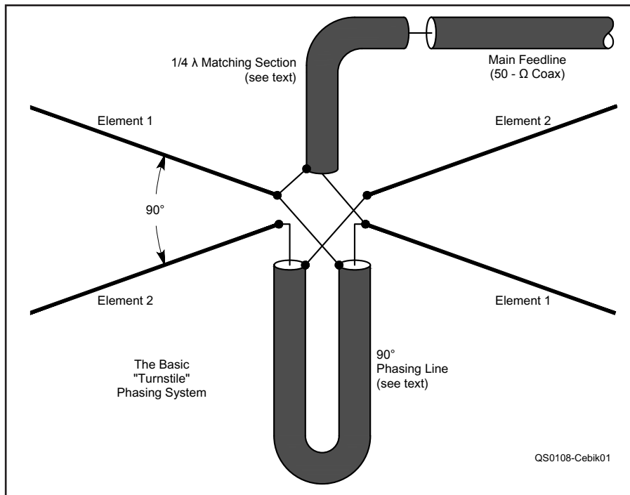
Fig 21.111 — The basic turnstile phasing (and matching) system for any antenna set requiring a 90° phase shift between driven elements in proximity.
