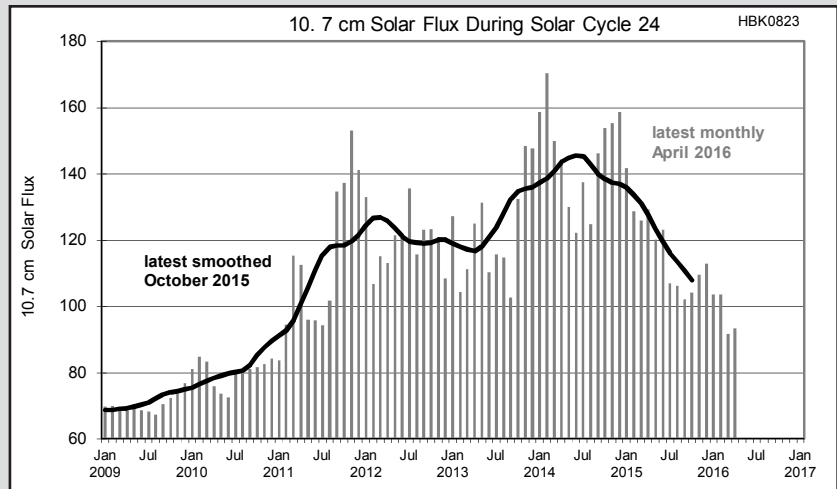
Figure 19.A1 — Monthly mean and smoothed 10.7 cm solar flux data through April 2016 and October 2015, respectively.
