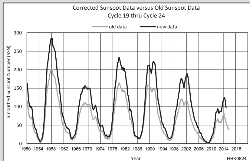
Figure 19.A2 — Corrected (see text) smoothed sunspot numbers and old smoothed sunspot numbers for Cycles 19, 20, 21, 22, 23 and 24.
