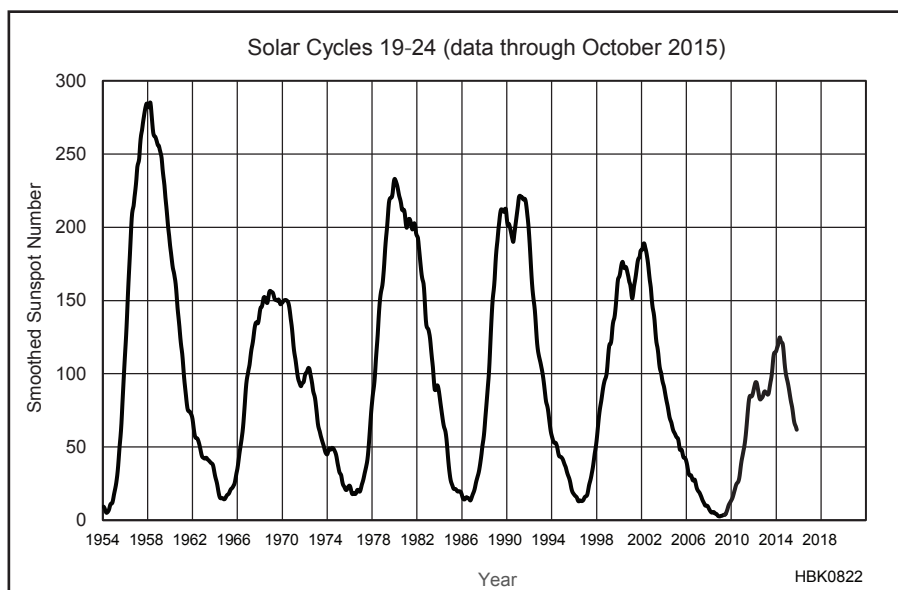
Fig 19.10 — Smoothed sunspot numbers (SSN) through October 2015 for solar cycles 19 to 24.
