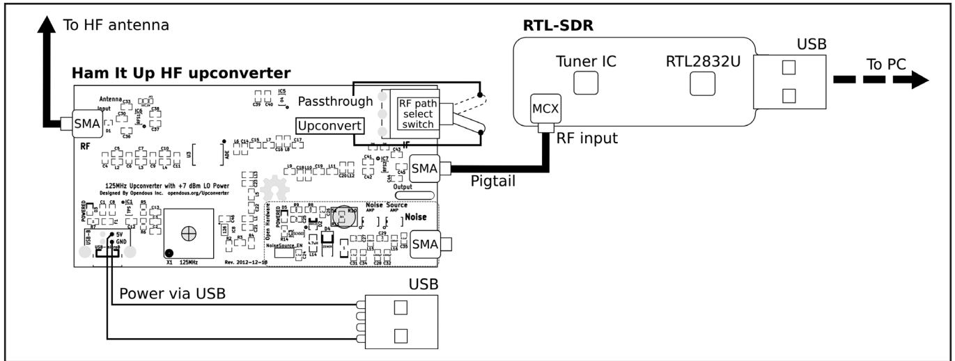
Fig 15.44 — Connecting an upconverter to the RTL-SDR dongle. The Ham It Up converter is shown as a typical example.
