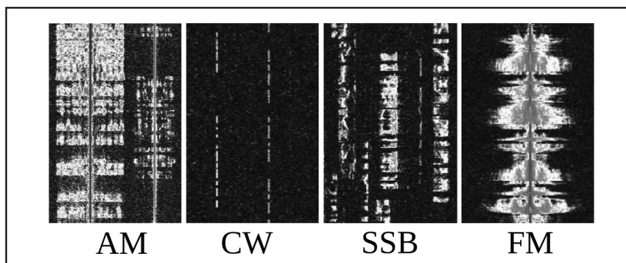
Fig 15.42 — Signals with different modulations on the waterfall display. Left to right — double-sideband, full-carrier AM, CW, single-sideband, and FM.
