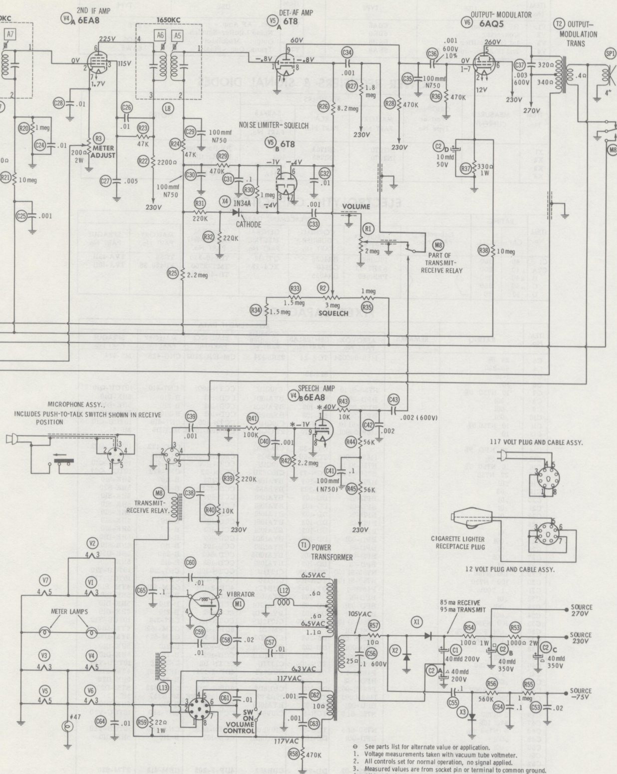
LAFAYETTE MODEL HE-20B
