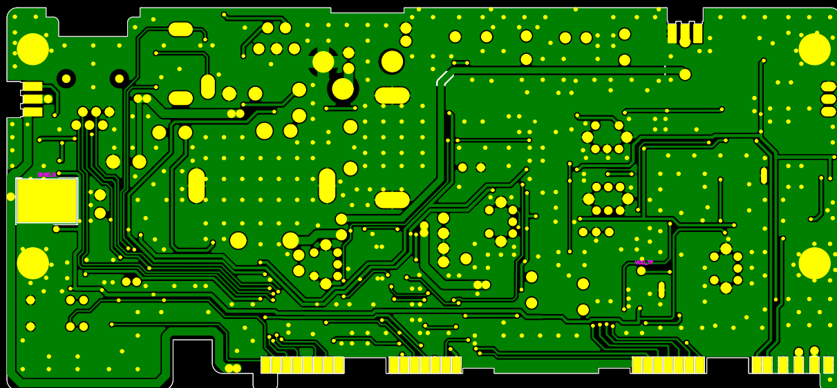
TX2720T SQ PCB VER 2.0
